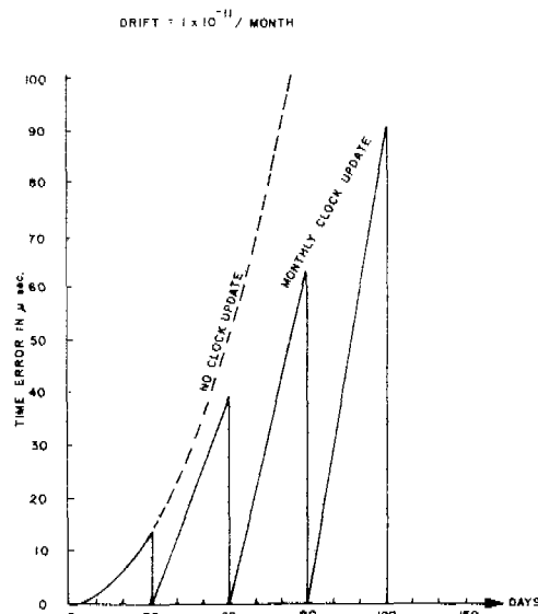
Figure 5. Rubidium Oscillator Drift
