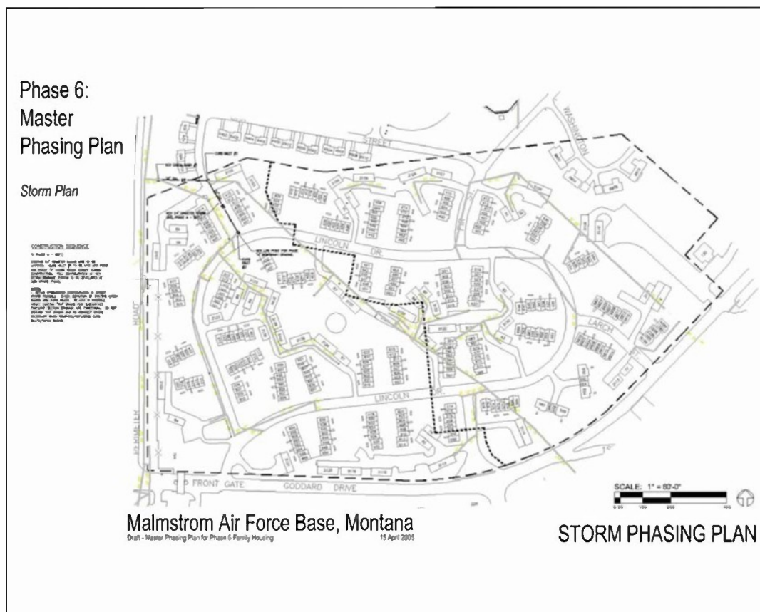
Figure 7 Storm sewer construction sequencing plan for Phase 6, Replace Family Housing Malmstrom Air Force Base, Great Falls Montana.
