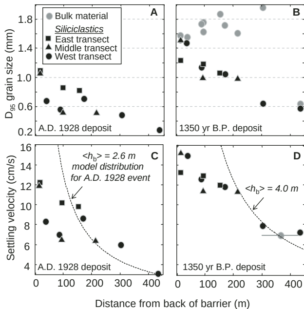
Figure 3. A–B: Shore-normal grain-size distributions measured for coarse fraction (>63 \mu\text{m} ) of A.D. 1928 and 1350 yr B.P. deposits. C–D: Particle settling velocities estimated for grain sizes shown in A and B. Black dashed line indicates distribution predicted by advective-settling model using 2.6 m and 4 m flooding depths estimated for the 1928 and the 1350 yr B.P. events. Gray line in D indicates the average settling velocity and maximum range that shell material was transported into lagoon.
