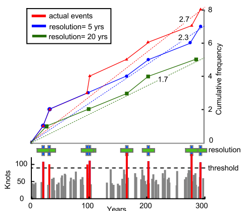
Figure 3. Example of synthetic overwash record. (bottom) A 300 year synthetic overwash record created for Vieques. Gray bars indicate maximum onshore winds recorded at the site using a random draw of synthetic storms. Red bars indicate storms which exceed the threshold (horizontal black dashed line) required for overwash to occur at the site. The blue and green bars above the wind reconstruction indicate discernable periods of overwash for temporal resolutions of 5 years and 20 years, respectively. (top) Actual (red) and discernable cumulative frequencies for a temporal resolution of 5 years (blue) and 20 years (green) for the synthetic overwash record in bottom plot. Numbers indicate the rate of resolvable overwash events per century based on the indicated temporal resolutions.
