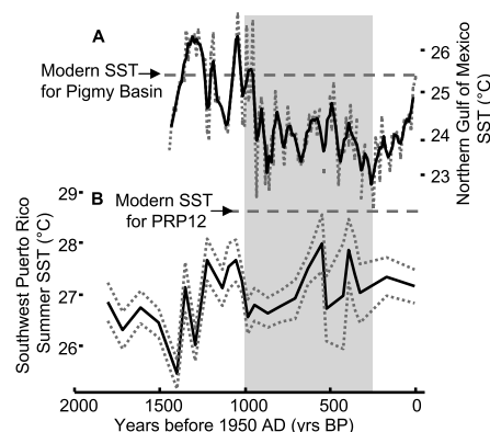
Figure 8. (a) Mg/Ca sea surface temperature (SST) reconstruction for Pigmy Basin in northern Gulf of Mexico [Richey et al. , 2007]. Markers represent individual measurements and solid line indicates three-point running mean. (b) Reconstruction of summer SSTs ~10 km offshore of southern Puerto Rico from core PRP12 (solid line) with 2σ uncertainties (dotted lines) [Nyberg et al. , 2002]. Dashed lines in Figures 8a and 8b indicate current SST estimates at each coring location. Discrepancies exist between the two SST reconstructions; however, both suggest a drop in temperature at ~1000 years B.P.
