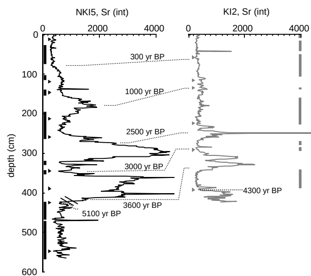
Fig. 7. Sr peak integrated area for cores NKI5 (black) and KI2 (gray) (See Fig.1 for locations). Thicker vertical lines indicate intervals with fine-scale (<1 mm) laminations. Solid arrows represent the depth of radiocarbon-dated samples from each core. Thin dashed lines indicates depths of equal age between cores based on the age model presented in Fig. 6.
