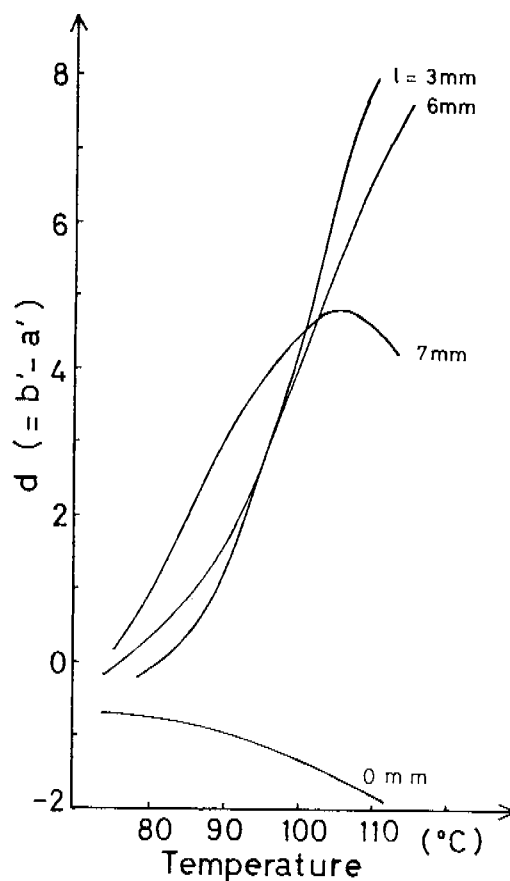
Fig.5 Values of d vs. temperature of the source, which are calculated from the experimental results.
