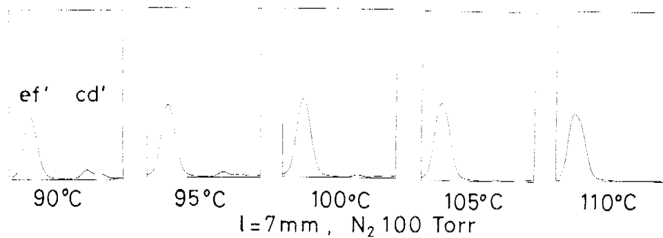
Fig.7 Calculated profile of the Rb-87 D-1 line from the composite-type pumping-light source.
