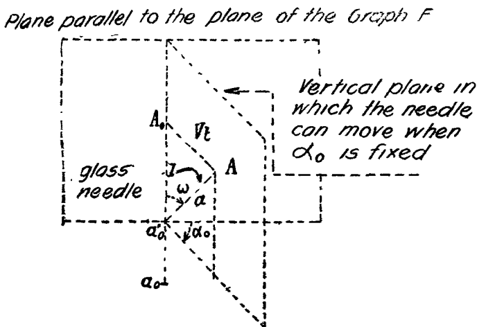
FIG. 8. TRANSMISSION OF THE VECTOR Vt TO THE GLASS NEEDLE
