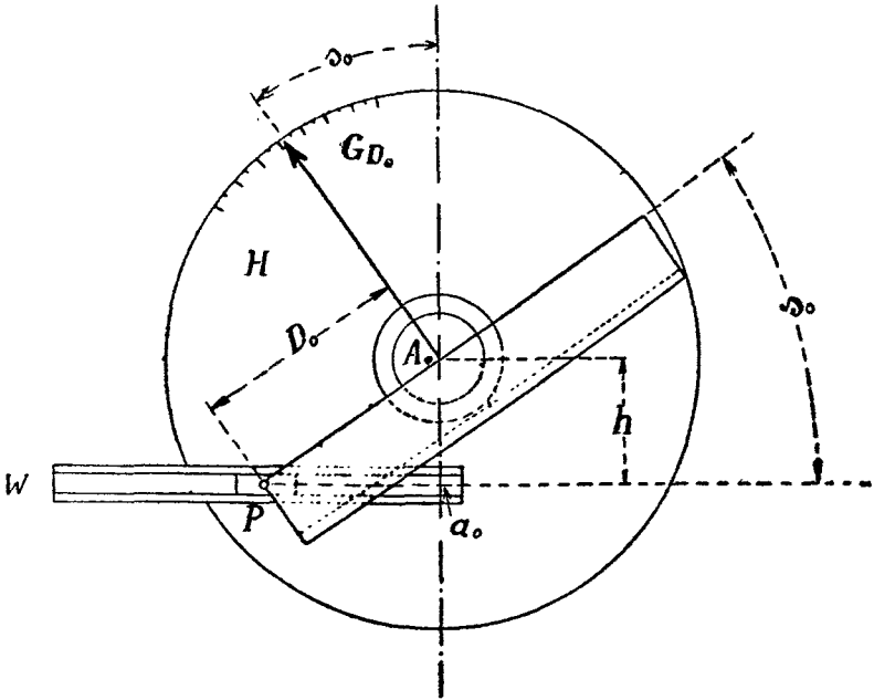
FIG. 3. THE AIMING TRIANGLE U
