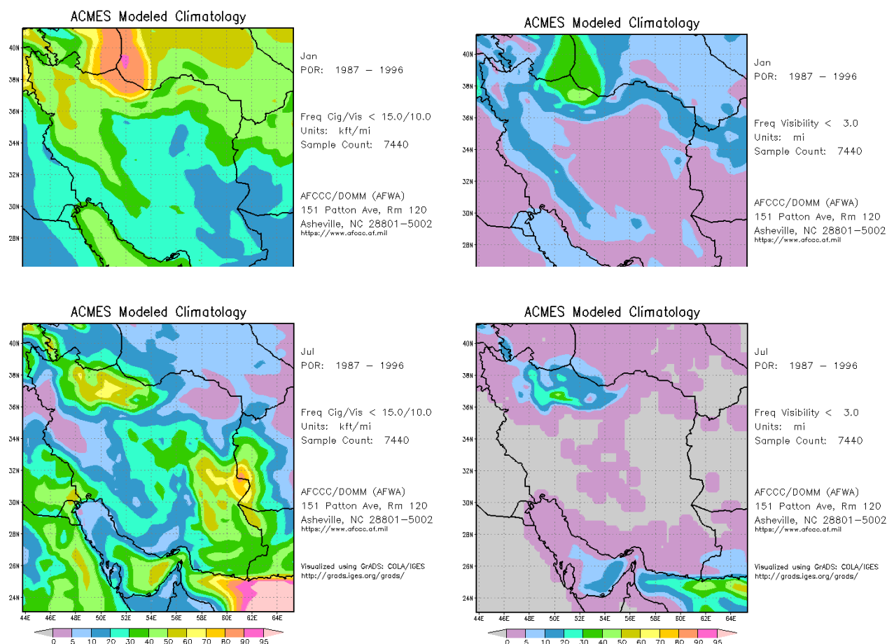
Figure 5-9: (left) - Ceilings below 15K and less than 10 miles horizontal surface visibility Figure 5-10: (right) - Horizontal surface visibility of less than 3 miles
