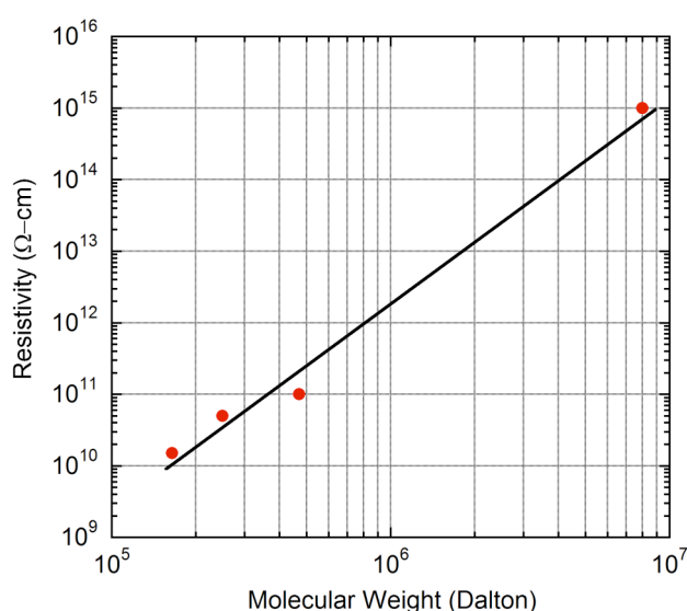
Fig. 2 (supplemental) Resistivity of DNA-CTMA spin-coated thin films as a function of DNA molecular weight.
