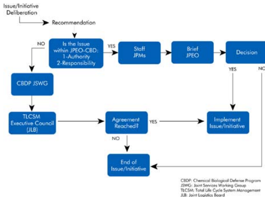
Figure 3-2. JLAC-CBD Process
