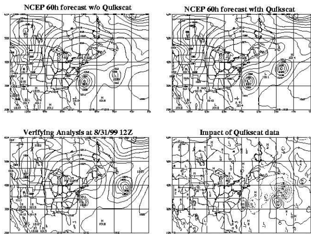
Fig. 7 Impact of QuikSCAT data in a test version of the NCEP operational environment. Verifying analysis is the lower left panel. Note the greatly improved position and depth of the mid- Atlantic storm. The magnitude of the impact is shown in the lower right panel.
