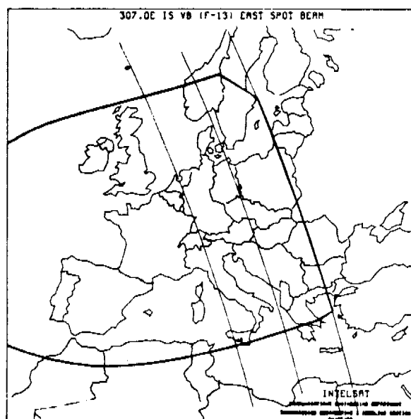
INTELSAT VA(1BS) East Spot Coverage from 307° East
