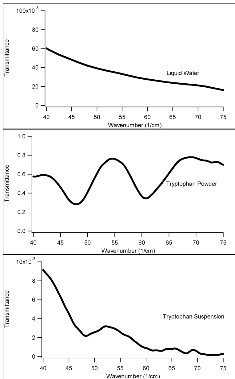
Figure 5. Terahertz transmittance spectrum of water, tryptophan powder and tryptophan suspension (0.74 gm/ml).
