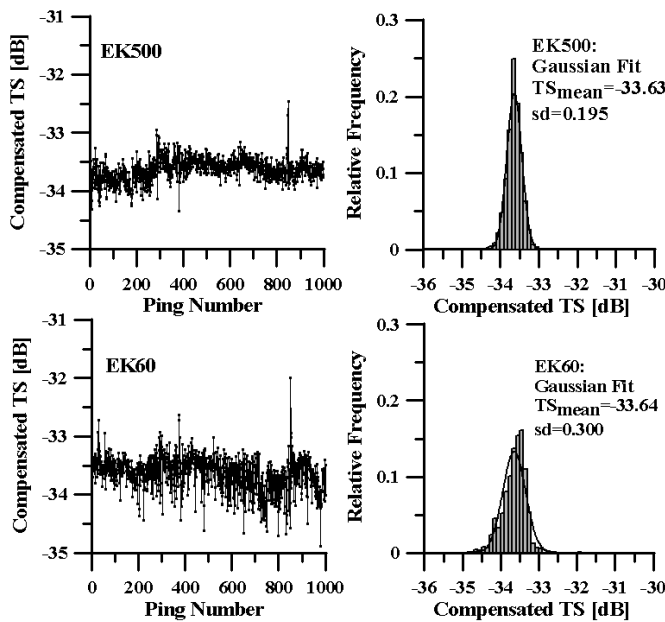
Figure 1. Time series (left panels) and split-beam target strength distributions (right panels) of on-axis echo amplitude measurements of a 60-mm-diameter copper sphere for the EK500 and EK60. Ping rate was 1 ping s^{-1} per echo sounder and 1000 pings represents approximately 17 minutes. Echo strength measurements were compensated for location in the acoustic beam to give split-beam target strengths. Mean split-beam target strength (TS) and standard deviation (sd) are derived from the Gaussian fit to the data [6].
