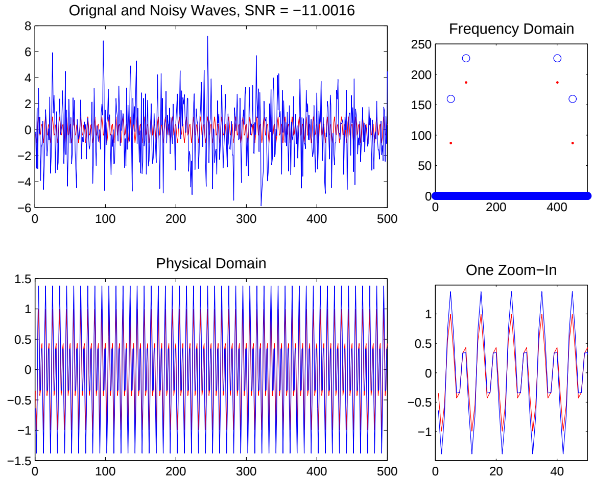
FIG. 7.4. Reconstruction using 80% random samples of \tilde{u} with \text{SNR} = -11.0016 . The upper left figure shows the original (red) and noisy (blue) signals; the upper right shows the reconstruction (blue circle) v.s. original signal (red dots) in Fourier domain in terms of their magnitudes (i.e. |\hat{u}^*| v.s. |\hat{u}| ); bottom left shows the reconstructed (blue) v.s. original (red) signal in physical domain; and bottom right shows one close-up of the figure at bottom left.
