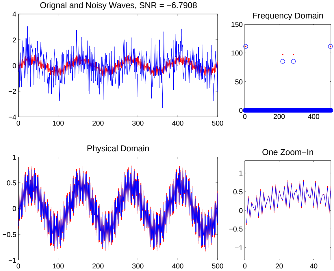
FIG. 7.3. Reconstruction using 60% random samples of \tilde{u} with \text{SNR} = -6.7908 . The upper left figure shows the original (red) and noisy (blue) signals; the upper right shows the reconstruction (blue circle) v.s. original signal (red dots) in Fourier domain in terms of their magnitudes (i.e. |\hat{u}^*| v.s. |\hat{u}| ); bottom left shows the reconstructed (blue) v.s. original (red) signal in physical domain; and bottom right shows one close-up of the figure at bottom left.
