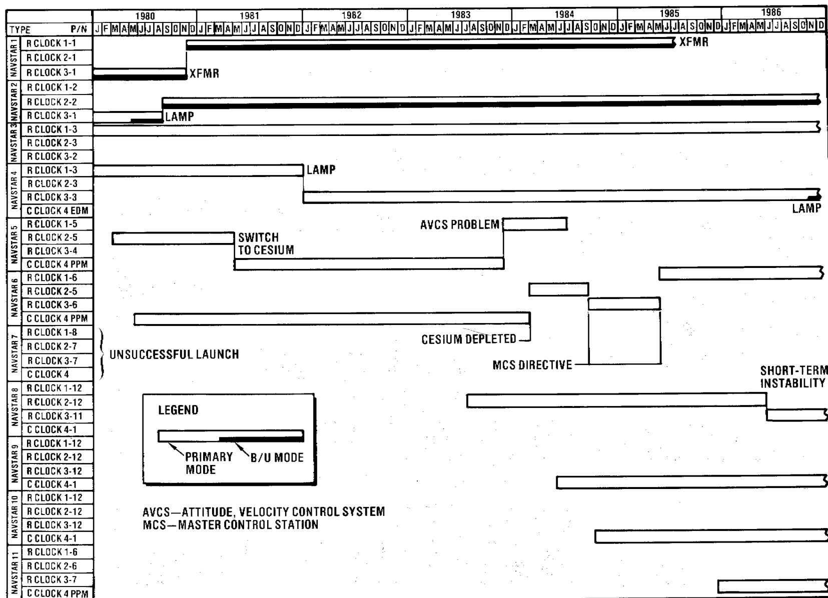
Figure 1. Navstar Clock Operating History
