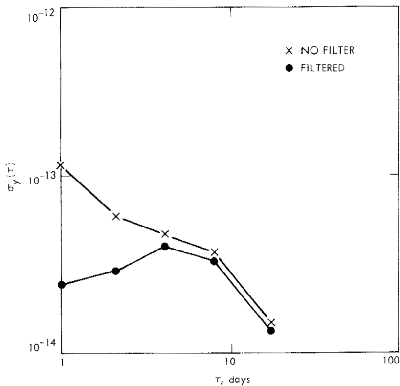
Figure 3. Allan Variances of Goldstone-UTC (NBS) Before and After Kalman Filter
