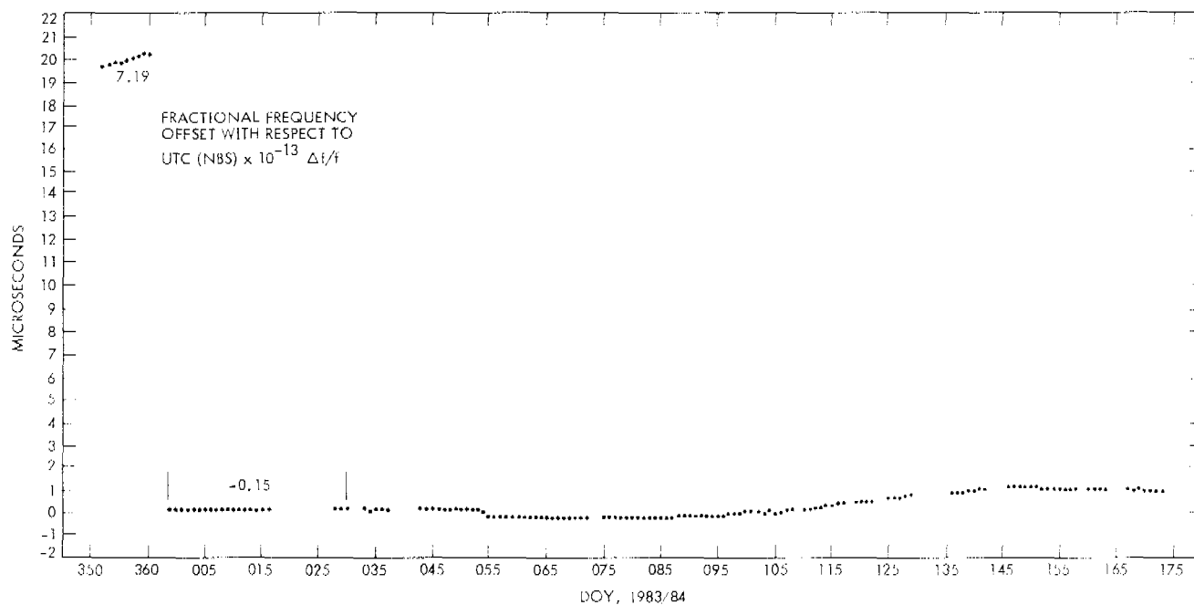
Figure 7a. Time Offset, Madrid versus UTC (NBS) Showing Frequency Adjustment and Clock Reset (Note the Different Ordinate Scale)
