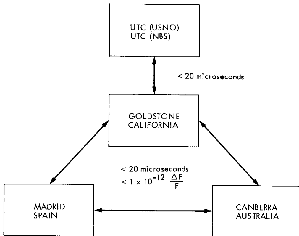
Figure 1. DFT System Functional Block Diagram
