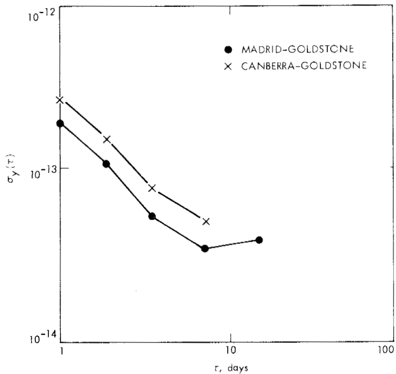
Figure 4. Allan Variances of Spain-California and Australia-California
