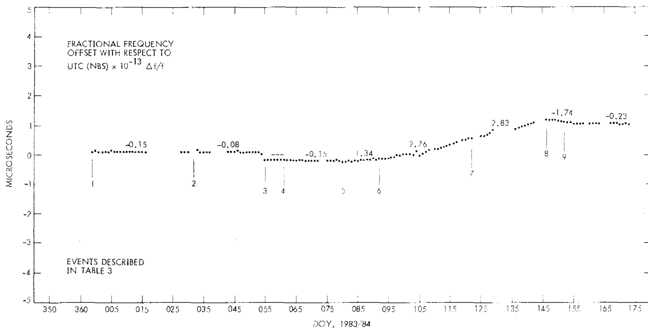
Figure 7b. Time Offset, Madrid versus UTC (NBS)
