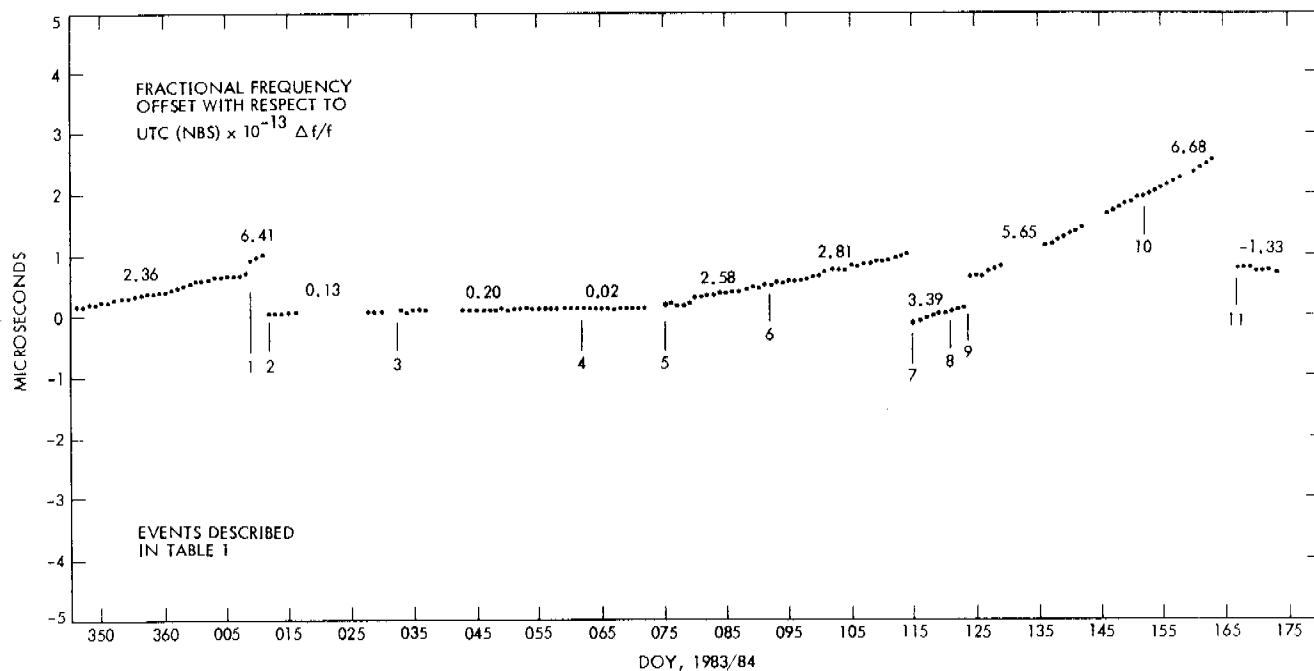
Figure 5. Time Offset, Goldstone versus UTC (NBS)
