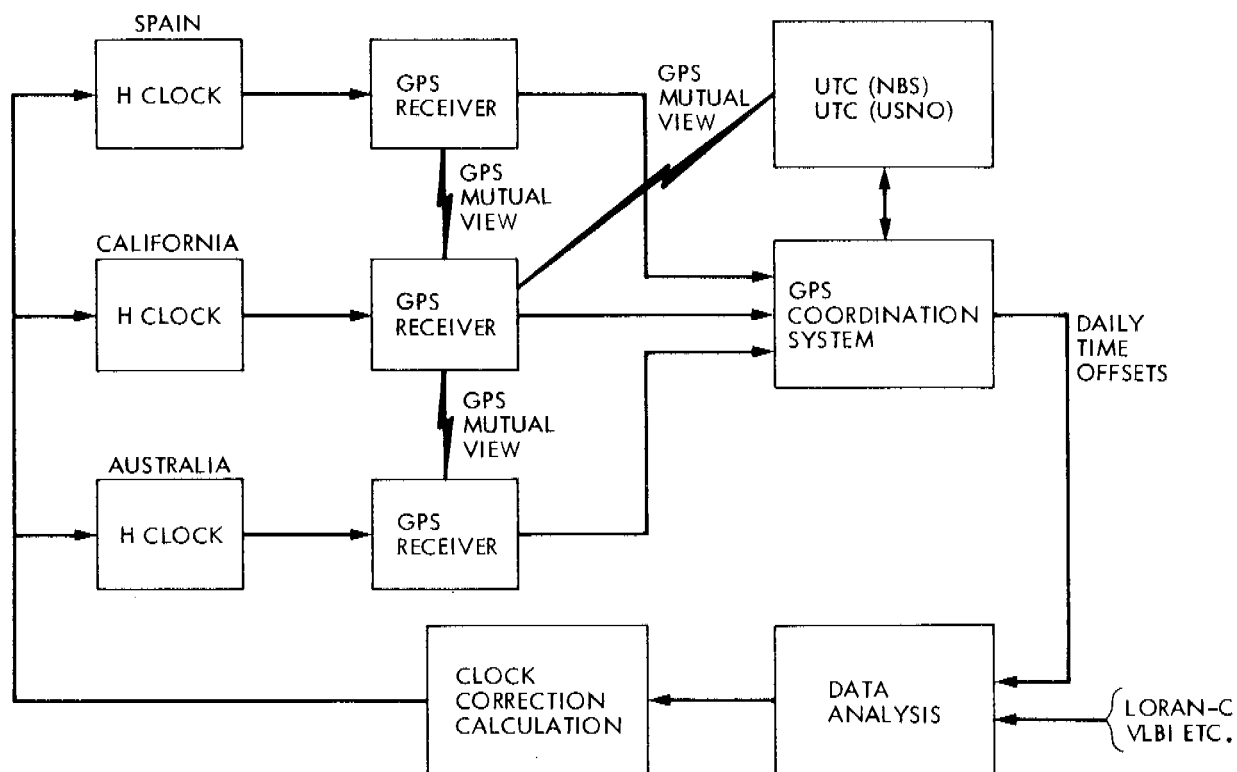
Figure 2. Frequency and Timing Control System
