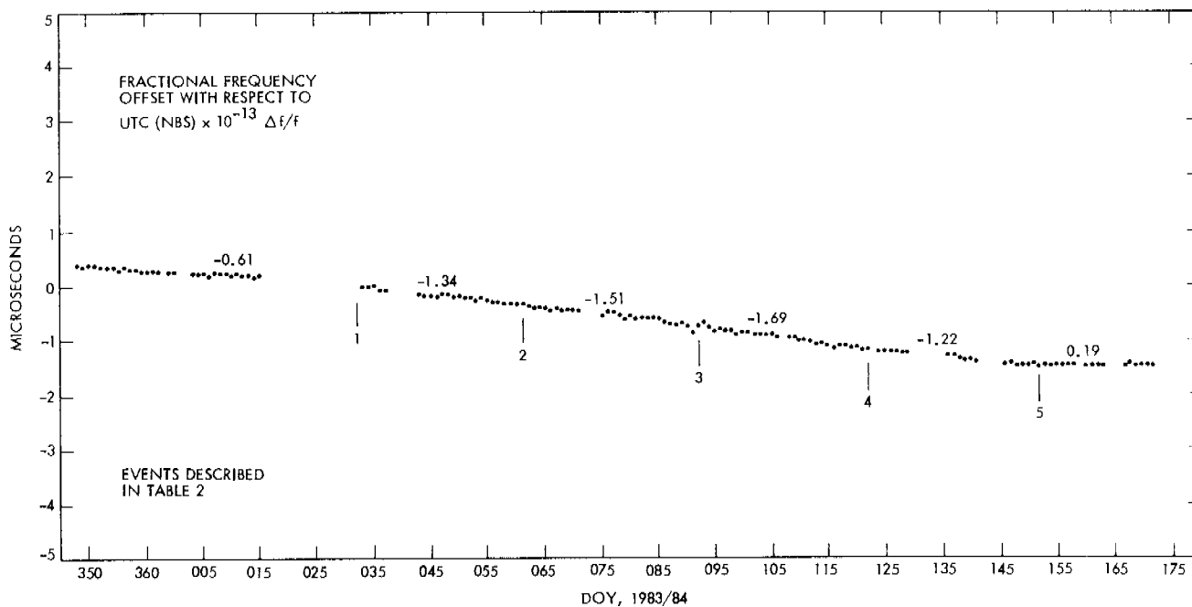
Figure 6. Time Offset, Canberra versus UTC (NBS)
