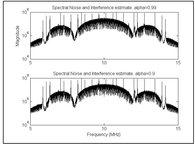
Fig. 3. Spectral interference estimate with \alpha = 0.9 .
