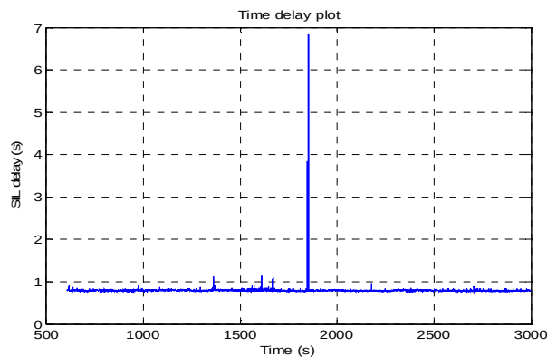
Figure 18. Plot of round trip delay between TSL and the SIL. Note that the state convergence solution recovered from the 7 second outage.
