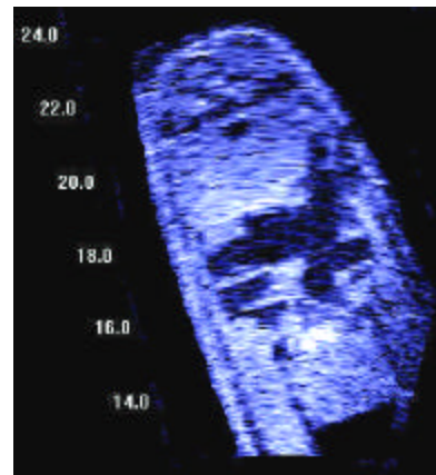
Fig. 8. A DIDSON image of the stern of vessel resting in 10 m of water. This image was taken in the low-resolution mode. The range scale is in meters.
