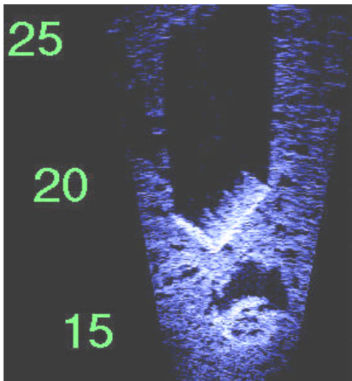
Fig. 4. A LIMIS image of a 50-gallon drum at 20 feet and an old tire at 15 feet.
