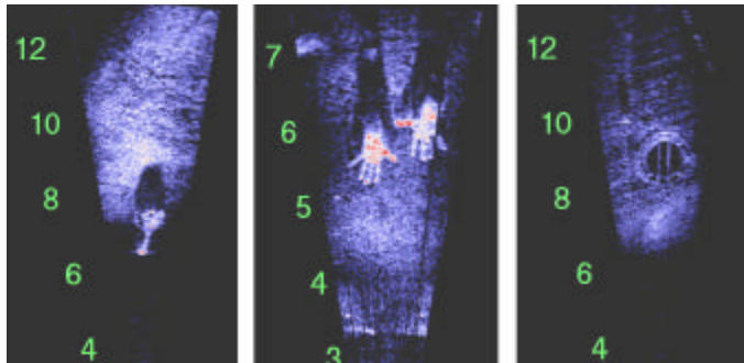
Fig. 5. Three sample images taken with the LIMIS. The left image shows a limpet mine on the hull of a ship 7 feet (2.1 m) from the sonar. The center image shows two hands. The right image shows an intake on the hull of a ship. The intake is approximately 46 cm in diameter and is 9 feet (2.7 m) from the sonar. The left and right images were taken in Chesapeake Bay in water with 15-cm visibility.
