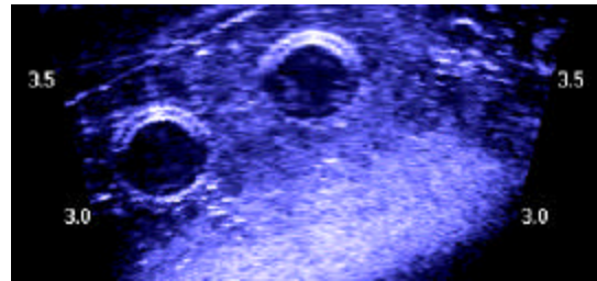
Fig. 11. A DIDSON image of the bottom of a metal pontoon showing instrumentation wells approximately 30 cm in diameter.
