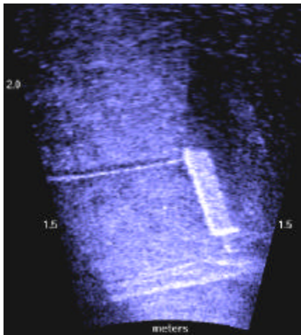
Fig. 7. A DIDSON image of an anode on a metal hull. This image was taken in the high-resolution mode. The range scale for DIDSON is in meters.
