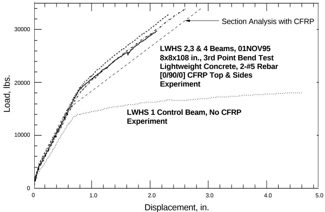
Figure 3. Load-Displacement Curves for LWS Series.
