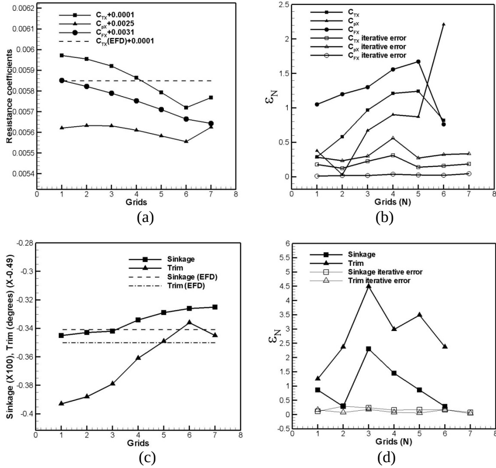
Figure 5. Verification for resistance and motions for Athena bare hull with skeg ( Fr=0.48 ): (a) resistance coefficients, (b) relative change \varepsilon_N = |(S_{N-1} - S_N)/S_i| \times 100 and iterative errors for resistance coefficients, (c) sinkage and trim, (d) relative change \varepsilon_N and iterative errors for sinkage and trim.
