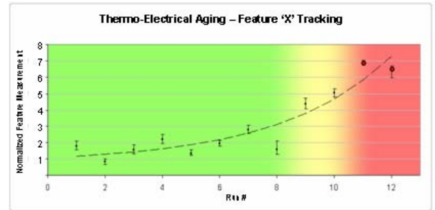
Fig 10: Feature Tracking of Thermo-Electrical Aging Process
