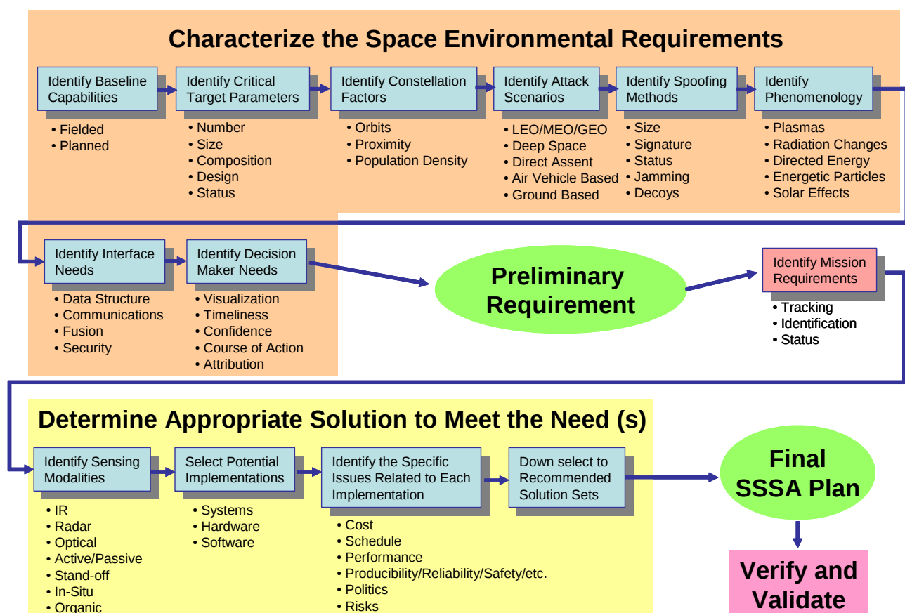
Figure 2: Process Model for Developing SSSA Solutions
