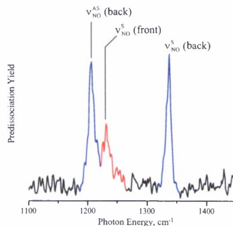
Figure 11: Isomer conversion spectra obtained by pumping \text{NO}_2^- \cdot \text{H}_2\text{O} on the OH stretch of the backside isomer near 3000 \text{ cm}^{-1} . The appearance of the frontside NO stretch at 1230 \text{ cm}^{-1} indicates successful conversion of the backside isomer to the frontside form.
