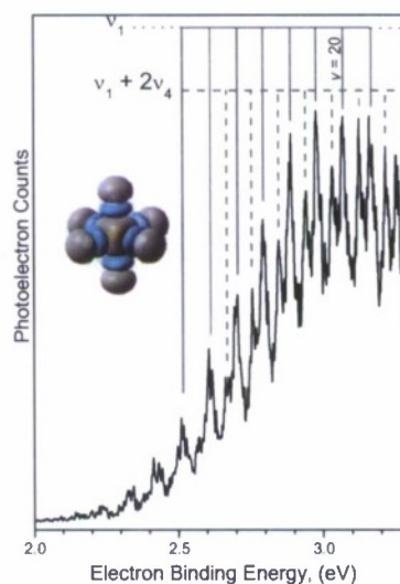
Figure 2: 355 nm photoelectron spectrum of SF_6^- \cdot Ar . The predominant vibrational feature is the 750\text{ cm}^{-1} ( \nu_1 ) symmetric stretch mode (solid lines), while the secondary progression is a combination of \nu_1 plus two quanta of the triply degenerate \nu_4 mode (dashed lines) (see Chem. Phys. Lett. 445 , 84 (2007)). The inset shows the SF_6^- excess electron orbital calculated at the B3LYP/aug-cc-pvdz level of theory.
