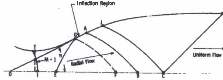
Figure 3: Radial Flow and Expansion Regions of Inviscid Contour[16]
