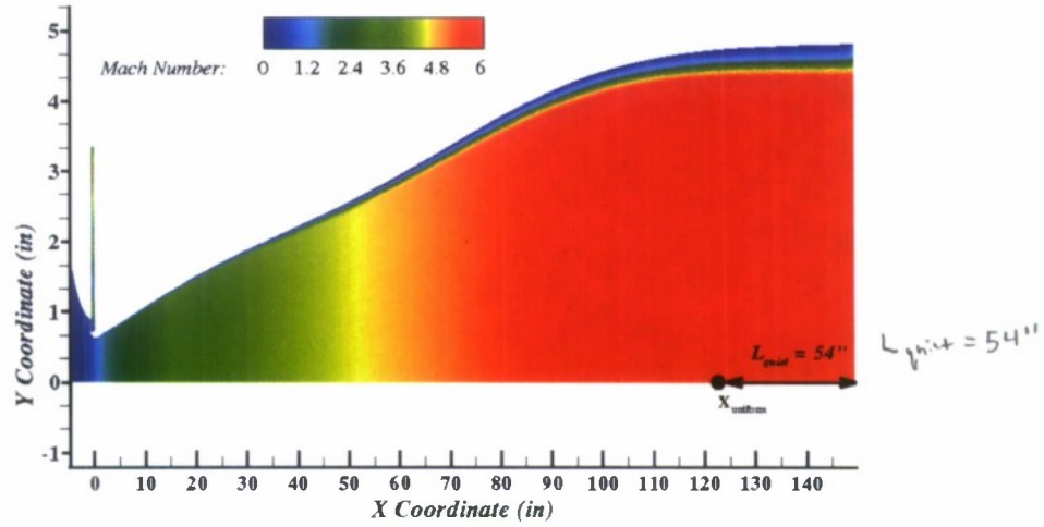
Figure 8: Optimal Design for Mach 6 Quiet Tunnel (vertical scale enlarged)
