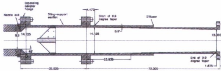
Figure 10: Expansion Section for Boeing-AFOSR Mach 6 Quiet Tunnel
