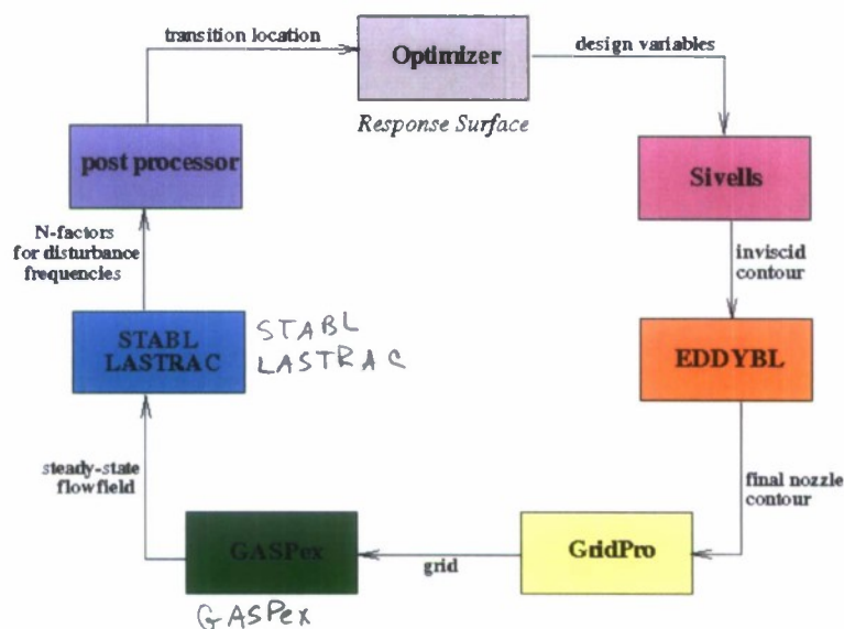
Figure 2: Automated Optimization Loop
