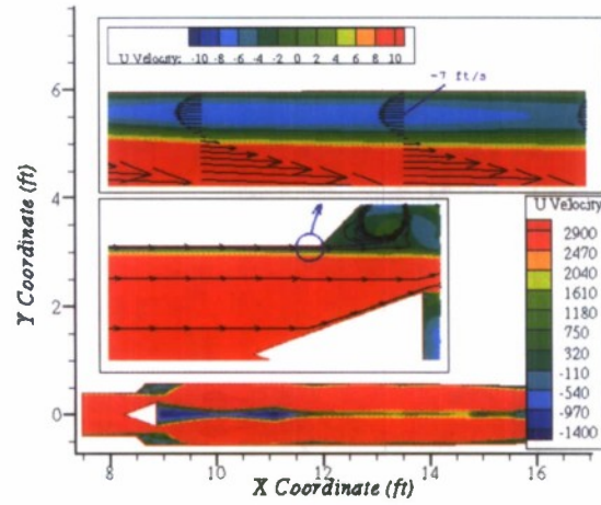
Figure 14: Streamwise Velocity Contours of Expansion Test Section with 20° Cone
