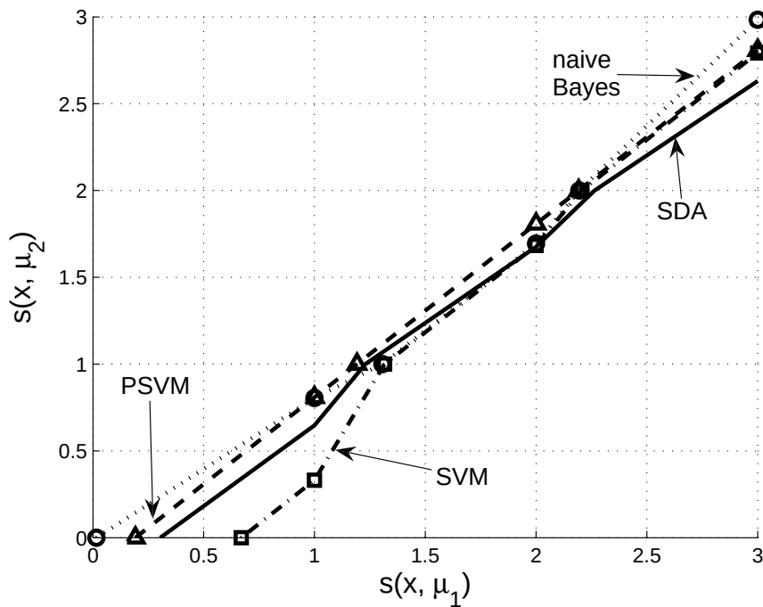
Figure 3.3: Class boundaries produced by SDA (-), SVM ( \square ), PSVM ( \Delta ), and naive Bayes (o) applied to the similarity.
