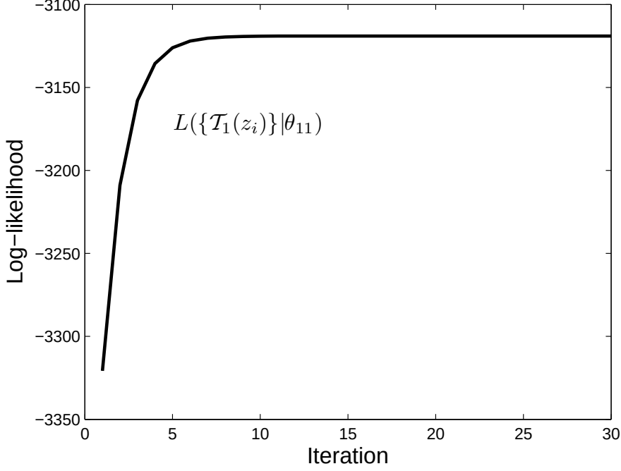
Figure 5.1: Log-likelihood of the training samples z_i \in \mathcal{X}_1 as a function of iteration number.
