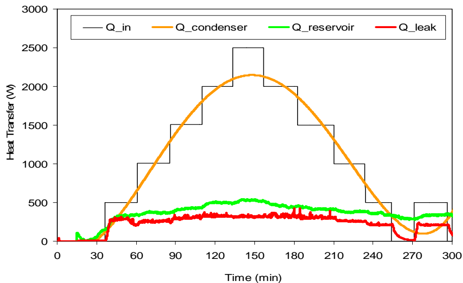
FIGURE 6. Calorimetry of hybrid two-phase loop.
