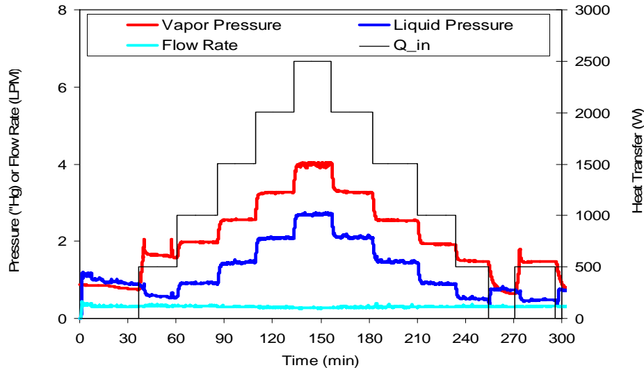
FIGURE 5. Pressure and liquid flow rate variations of hybrid two-phase loop vs. heat input.
