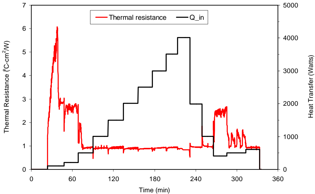
FIGURE 9. Thermal resistance variations of evaporator of hybrid two-phase loop vs. heat input.
