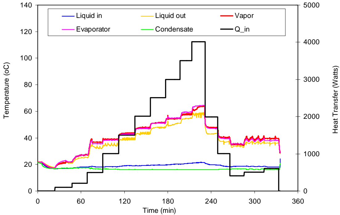
FIGURE 8. Temperature variations of hybrid two-phase loop vs. heat input.
