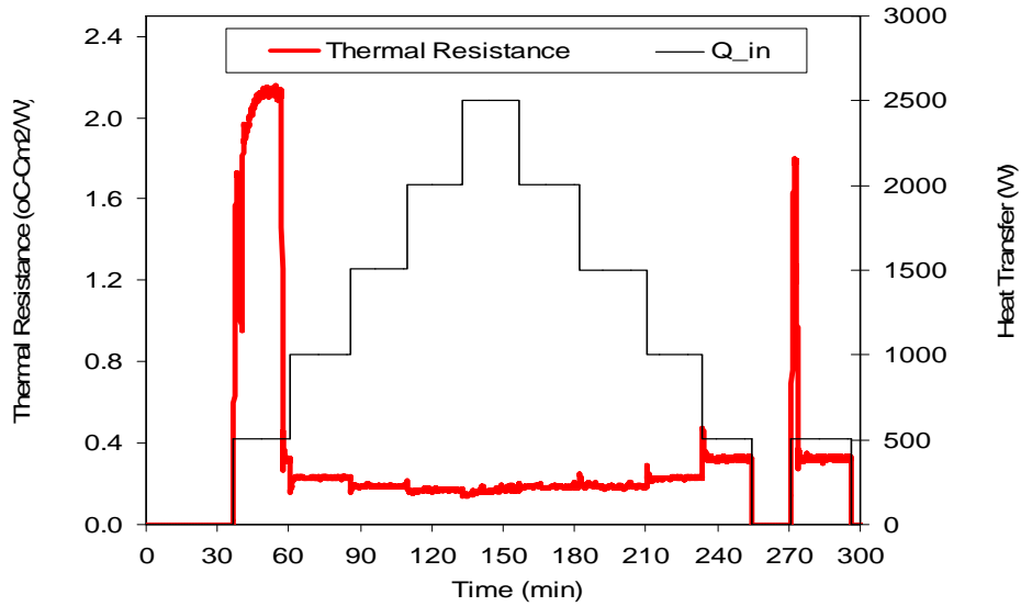
FIGURE 7. Thermal resistance variation of evaporator of hybrid two-phase loop vs. heat input.
