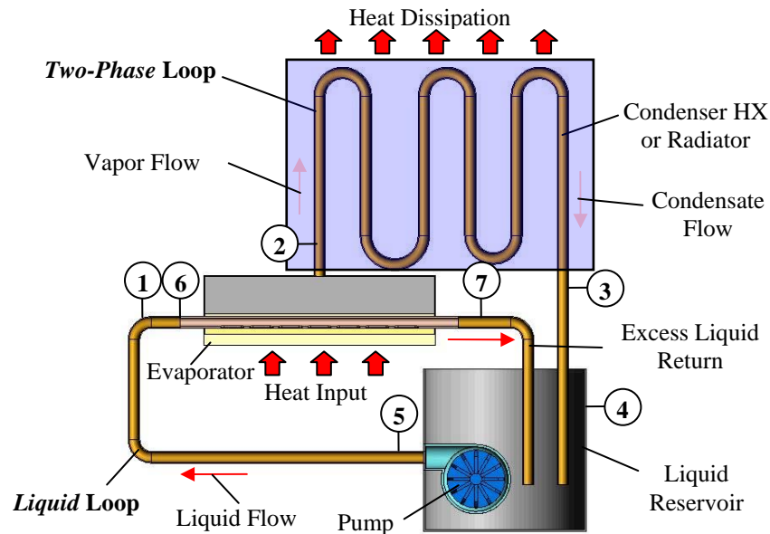
FIGURE 1. Schematic diagram of hybrid two-phase loop.
