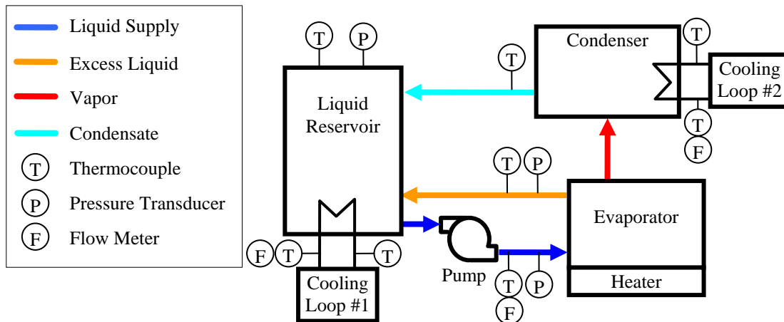
FIGURE 3. Schematic of hybrid two-phase loop with single evaporator.
