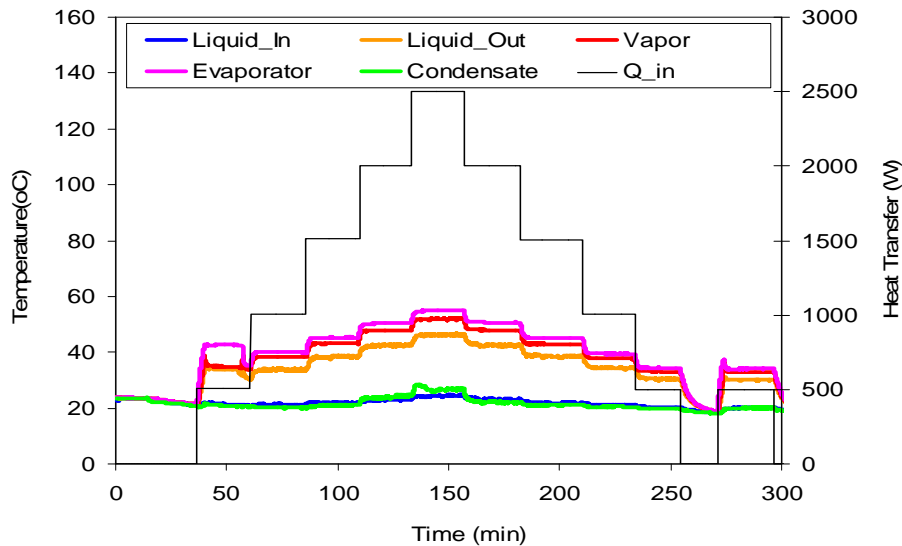
FIGURE 4. Temperature variations of hybrid two-phase loop vs. heat input.
