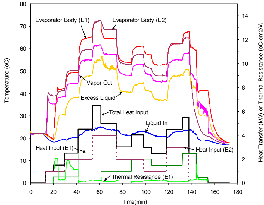
FIGURE 10. Thermal test results of dual-evaporator hybrid two-phase loop.
