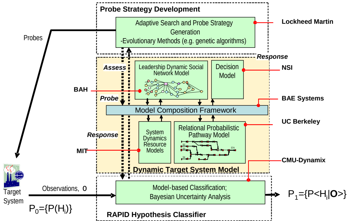
Figure 1: PAINT Architecture
