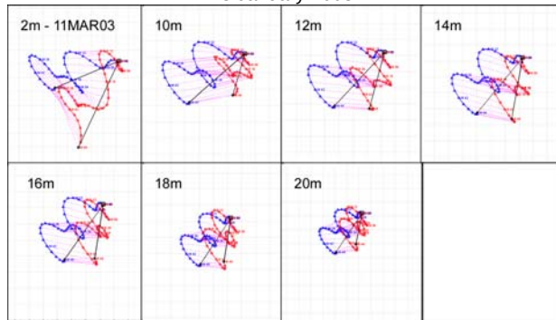
Fig. 6.b. Same as Fig. 6.a. for 11 March 2003.
