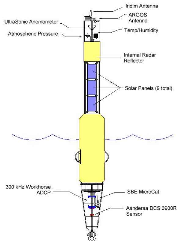
Fig. 1. TABS schematic.
