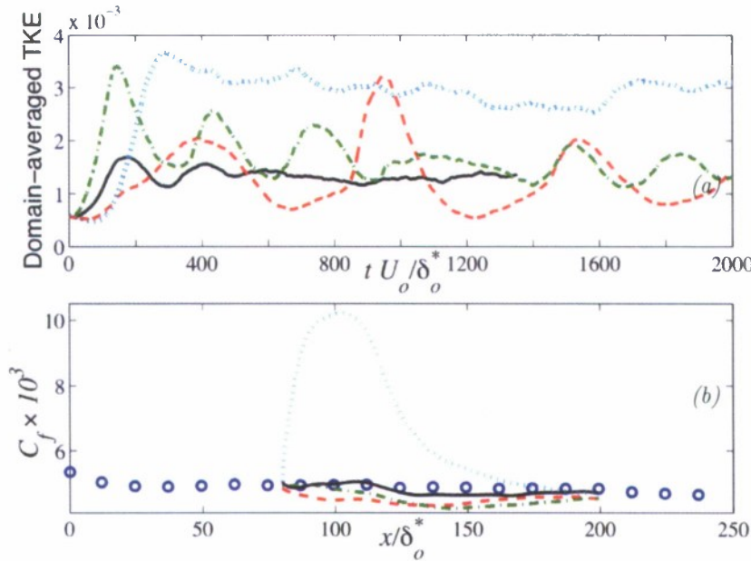
Figure 4: (a) Domain-averaged turbulent kinetic energy for \cdots T_{ave} = 1, K_I = 5, K_P = 30 ; \text{—} T_{ave} = 10, K_I = 5, K_P = 30 ; --- T_{ave} = 100, K_I = 1, K_P = 1 ; - \cdot - T_{ave} = 100, K_I = 5, K_P = 30 . (b) C_f for the reference LES ( \circ ) and the cases shown in (a).
