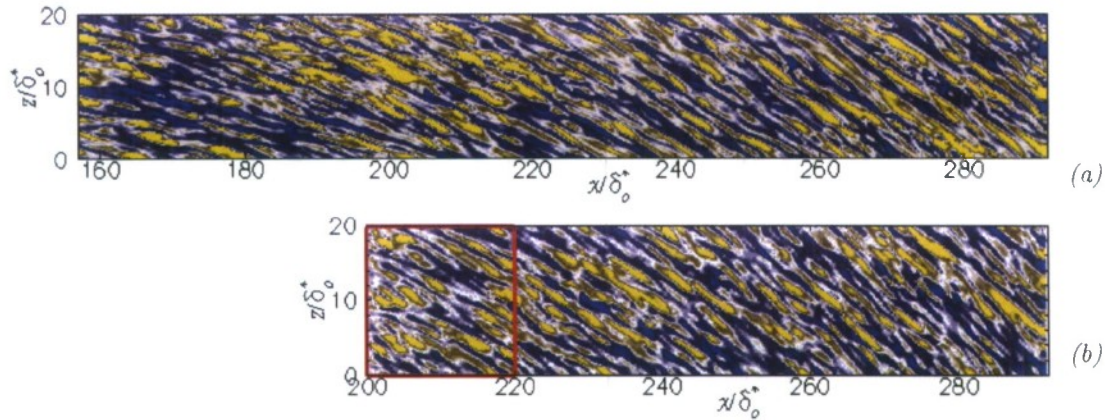
Figure 15: Contours of streamwise velocity fluctuations in a xz -plane near the wall, y/\delta^*/o = 0.18 . (a) Reference LES (only part of the domain is shown); (b) hybrid RANS/LES.
