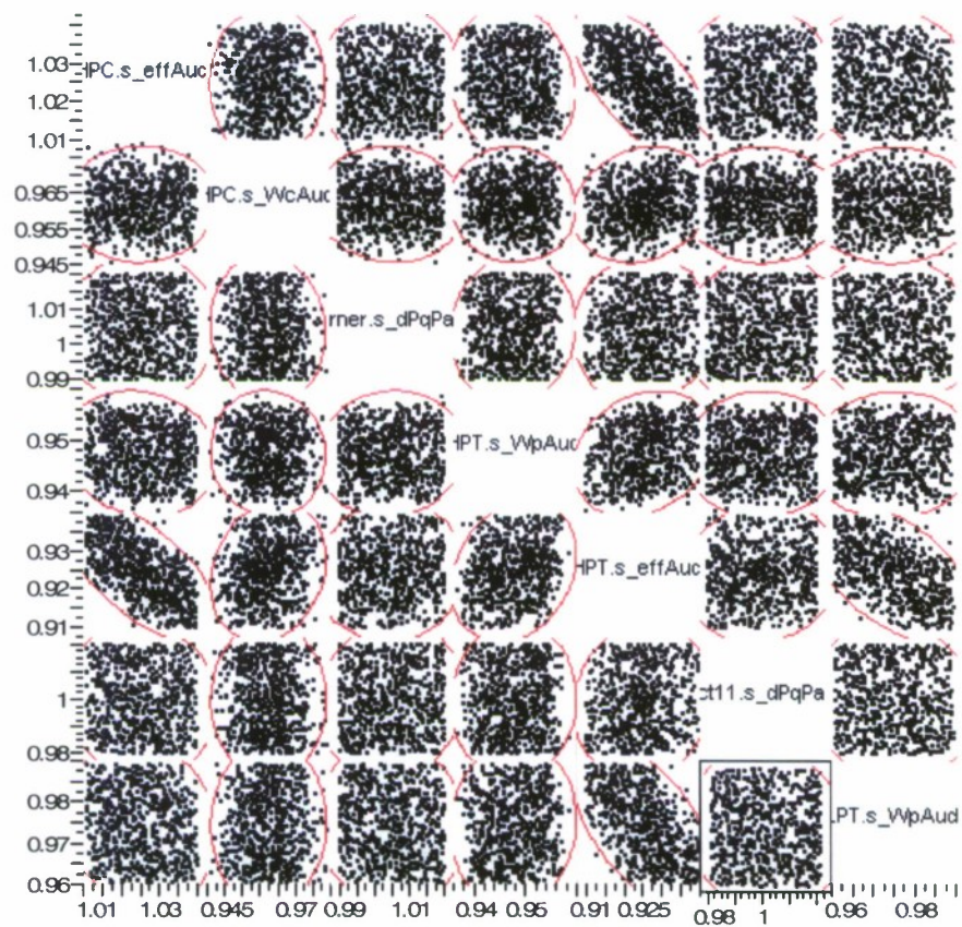
Figure 18: Correlation Plots
