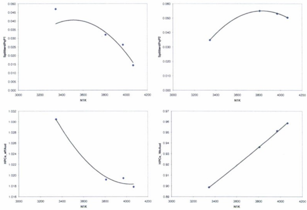
Figure 14: Modifier curve fits for Splitter and HPC
