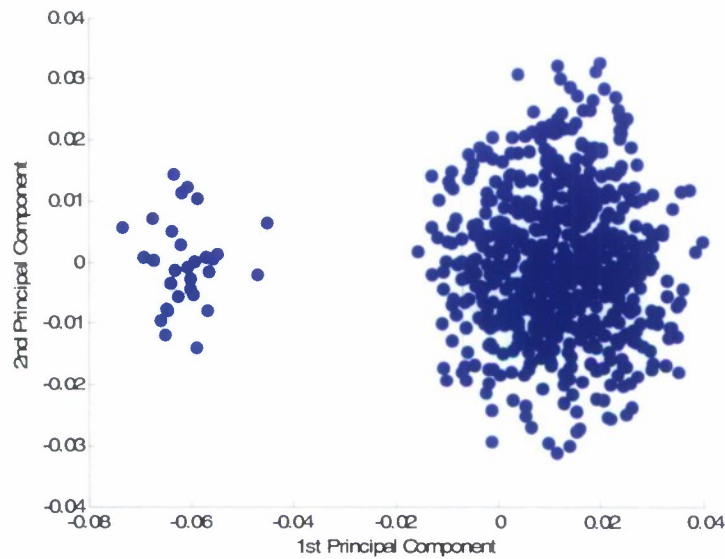
Figure 19: Projected Data onto the Principal Component Space
