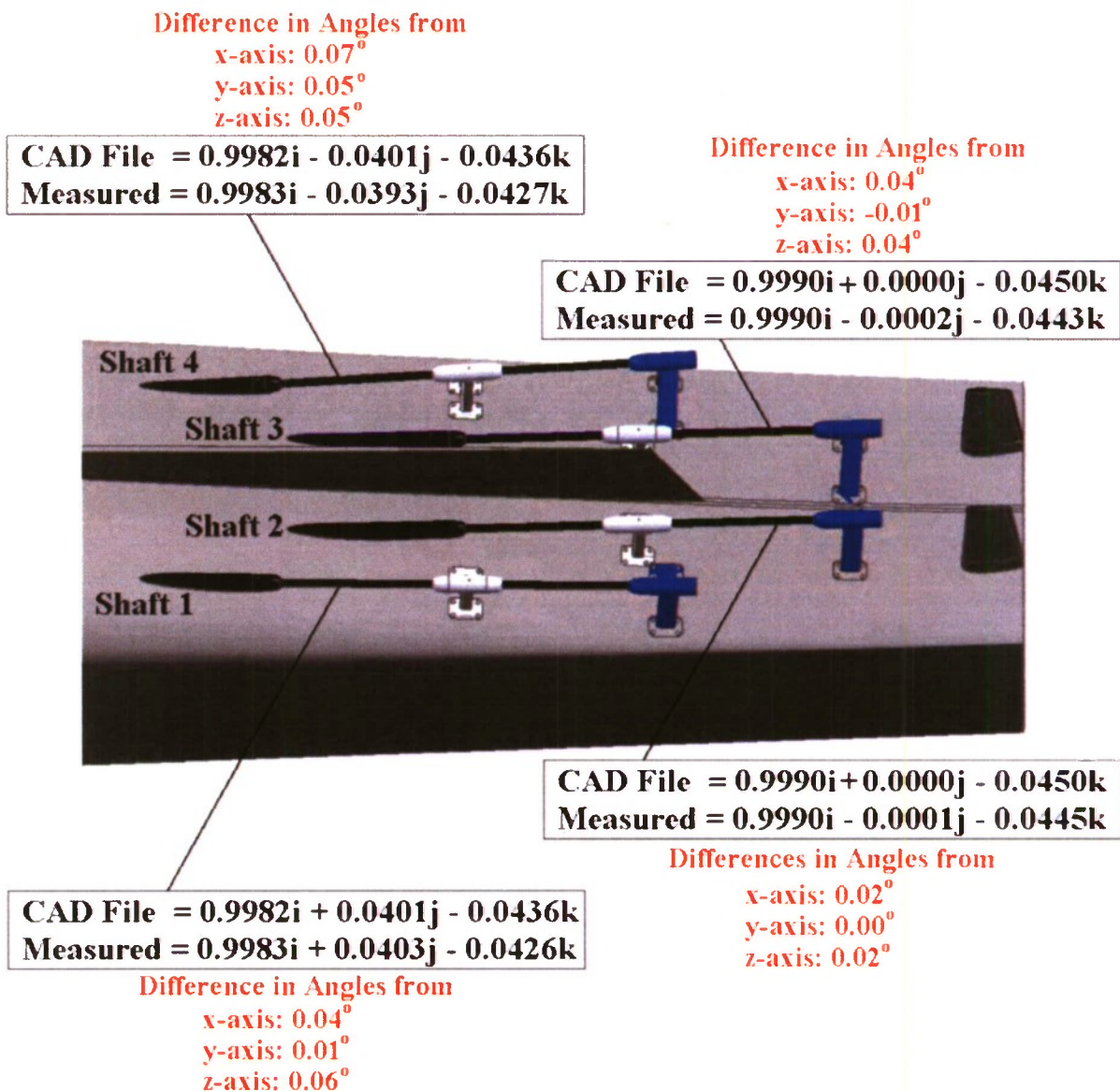
Figure C12. Design and Measured shaft vectors with their corresponding angle difference from the axis
