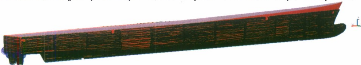
Figure C1. Model 5653 point cloud data superimposed on CAD surface.
