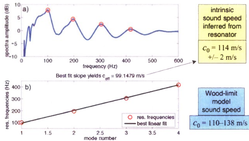
Fig. 2. (Color online) The resonator spectrum obtained for the kaolinite sediment. The four lowest resonance frequencies are identified with circles. (b) The effective sound speed c_{eff} inside the gassy kaolinite-filled waveguide is inferred from these frequencies, where a least-squares fit yields c_{eff} = 99.1 m/s. After correcting for the elastic waveguide effect, the intrinsic sound speed inferred from the measurements was c_0 = 114 m/s \pm 2 m/s, where the range is due to finite spectral resolution and the uncertainty in the resonator length L . The Wood limit model [Eq. (1)] predicted c_0 = 110-138 m/s, where the range is due to the uncertainty of the void fraction.
