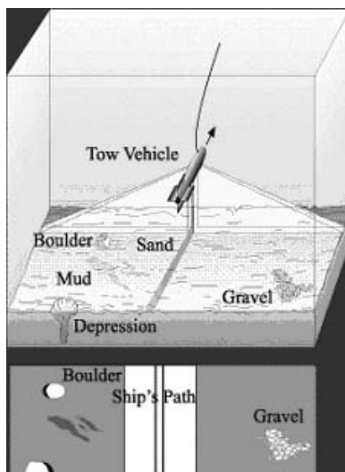
Figure 1. Illustration of a towed sidescan sonar system with resulting sidescan sonar imagery.
