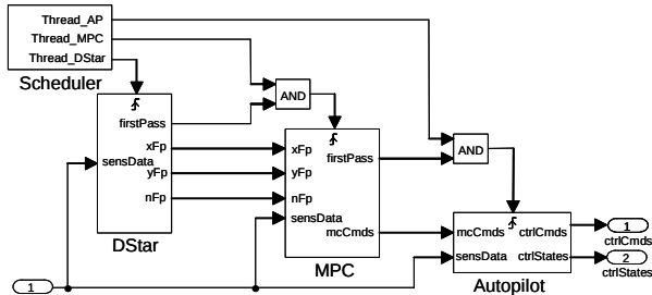
Fig. 2: Vehicle Control System
