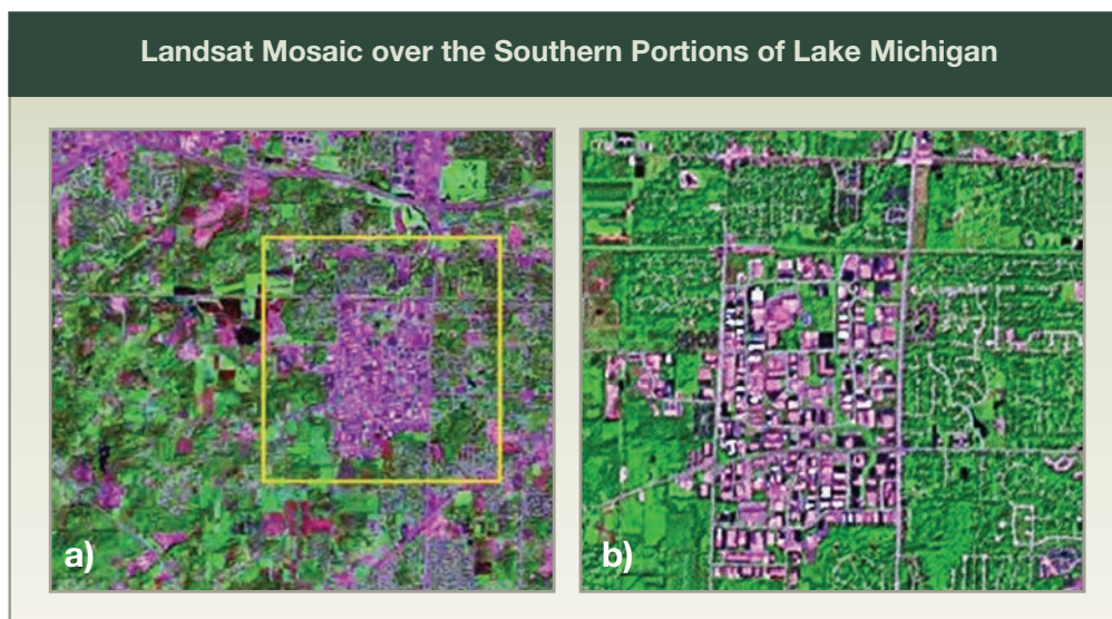
Figure 21: Landsat Mosaic over the Southern Portions of Lake Michigan. Landsat mosaic products over the southern portions of Lake Michigan and adjacent areas of the United States: (a) a full-resolution 28.5-m 2 subset for the circa 1990 epoch; and (b) a full-resolution 14.25-m 2 subset of the circa 2000 epoch. These are examples of the data available globally from NASA's Global Ortho-Rectified Landsat Data Set. Credit: C.J. Tucker, NASA/ Goddard Space Flight Center.
