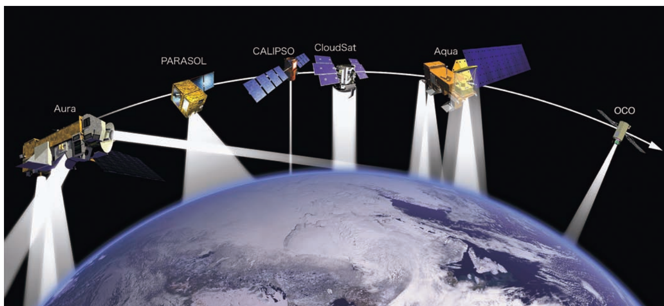
Figure 43: The "A-Train." This figure illustrates the constellation of satellites known as the "A-Train," which are making nearly contiguous observations of many facets of the Earth system. Credit: NASA.
