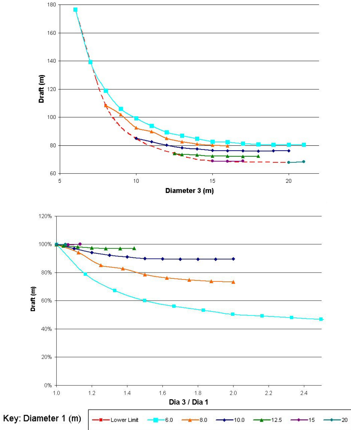
Figure 4 - Spar Diameter vs. Draft Results
