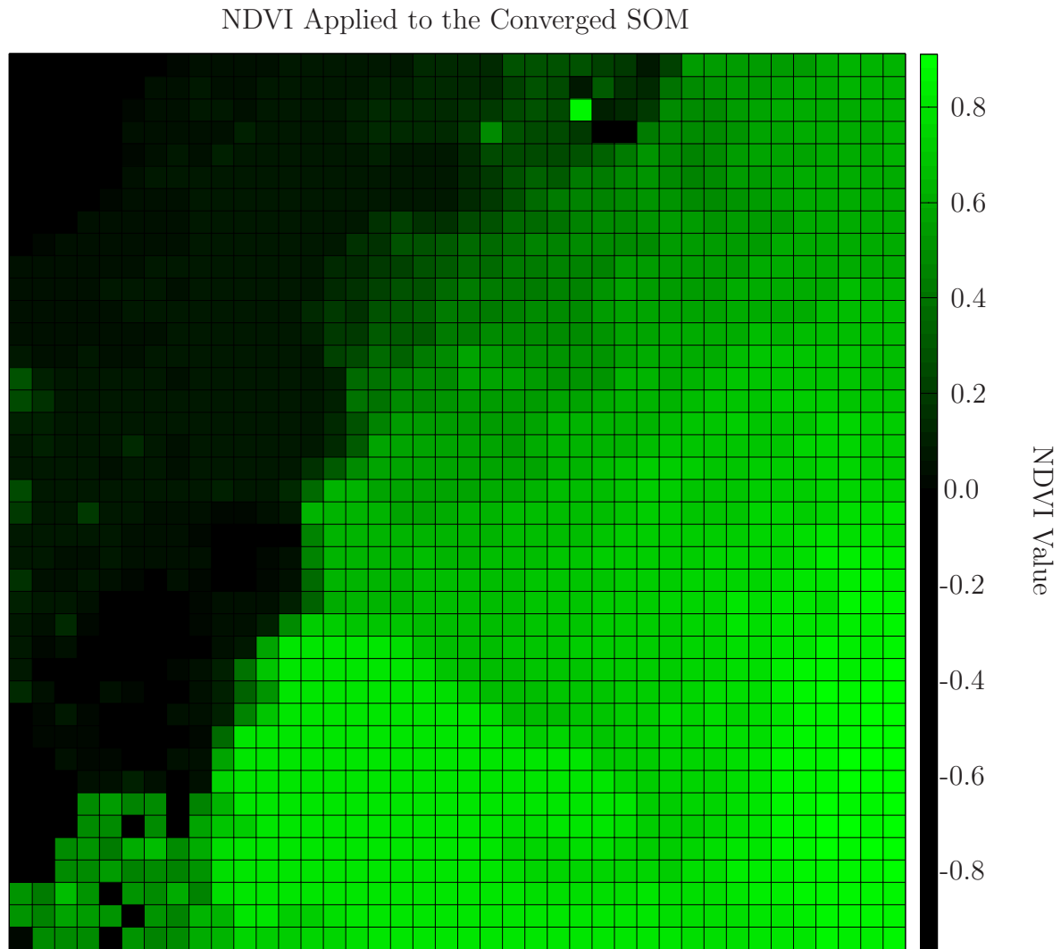
Figure 4.3: The result when NDVI is applied to the converged SOM from Figure 4.2. The color map has been adjusted to fade from green to black at the lower limit of confidence, \text{NDVI} > 0.3 . The brighter the pixel, the higher the confidence that it is vegetation.
