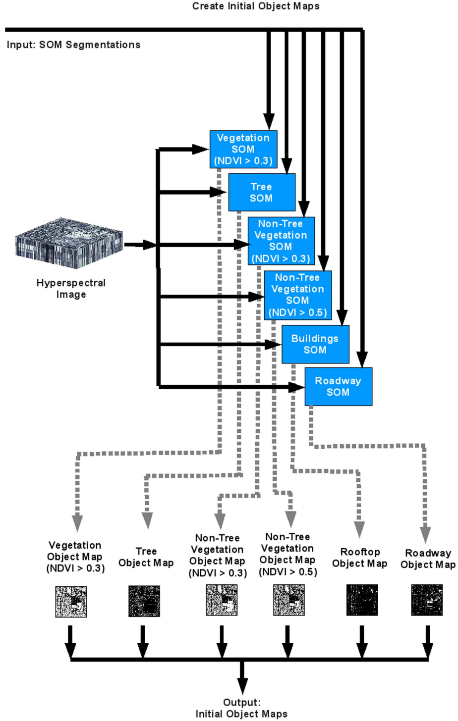
Figure 3.10: This is the process flow diagram for the create the initial object maps step. The nearest neighbor PE (in the \ell_2 -norm sense) for each SOM segmentation is located for each sample pixel of the hyperspectral image. The spatial location of the sample pixel is marked with the binary “true” or “false” in the corresponding initial object map , depending on the binary state of the SOM segmentation . One example SOM segmentation is shown in Figure 3.11.
