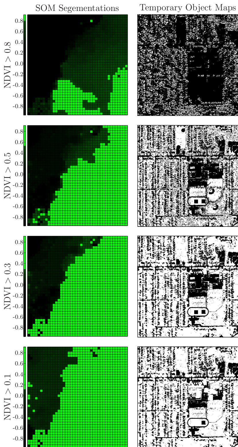
Figure 4.5: Each of the vegetation SOM segmentations (left column) are processed into temporary object maps (right column) using the process from Figure 3.11. Green PEs and white pixels are binary “true” indicating the presence of vegetation. The top right object map does not encompass the vegetation, and the bottom right object map marks the large building in the center of the image as vegetation.
