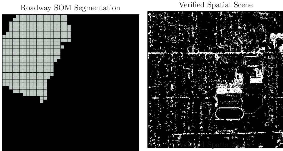
Figure 4.10: Exemplar spectra chosen with the process shown in Figure 3.8 in combination with spatial scene verification are used to set a \ell_2 -norm threshold resulting in the roadway SOM segmentation (left image). During spatial scene verification, the threshold is adjusted while verifying the results in the spatial object map (right image). The grey PEs and white pixels are “roadway” and the black PEs and pixels are “not roadway”.
