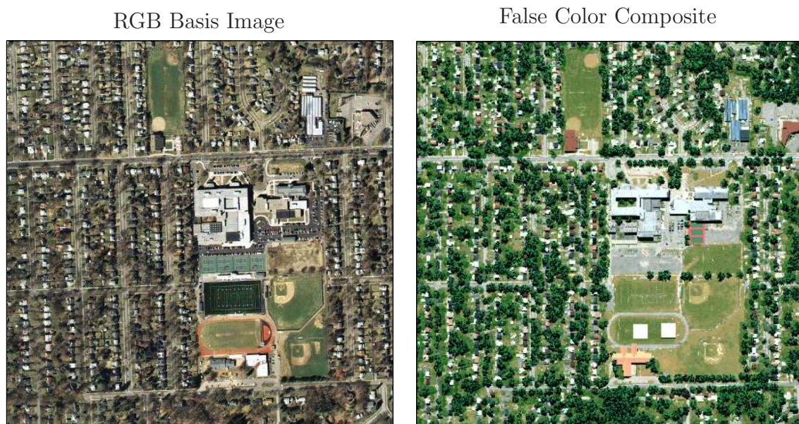
Figure 4.1: The satellite RGB image (left) is compared to the false color composite image (right) of the hyperspectral image. The satellite image was used as a layout reference to create the layout of Megascene1, from which the hyperspectral image is generated. The similarities and differences are discussed in Section 4.1.0.3.
