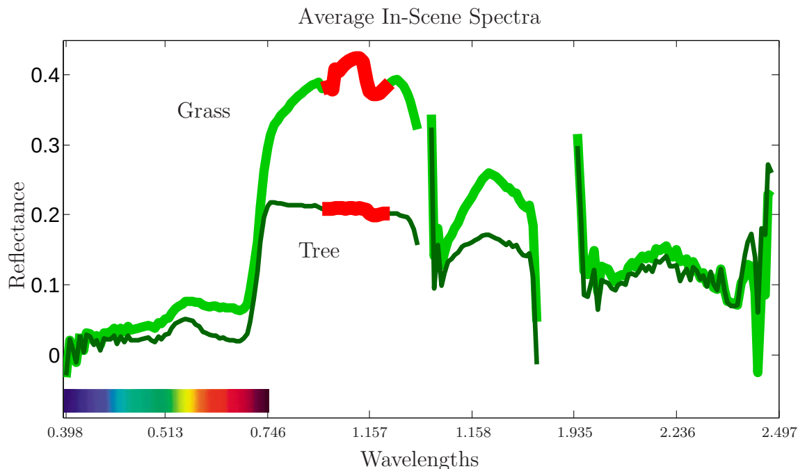
Figure 3.6: Trees are identified using the NIR scatter tree identification region (thick red line) between wavelengths 0.951\text{--}1.247\mu\text{m} . Urban grass (light green line) exhibits a larger amount of NIR scatter than maple tree leaves (dark green line). This variation is exploited to segment the “tree” neighborhood of the SOM.
