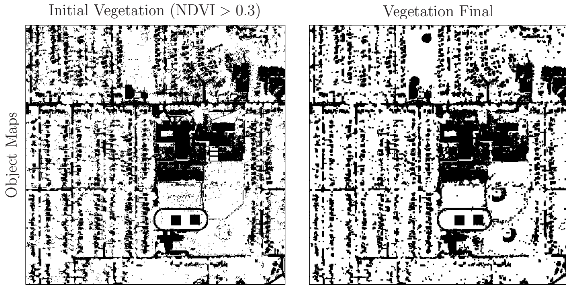
Figure 4.12: A comparison between the “vegetation ( \text{NDVI} > 0.3 )” initial object map (left image), which undergoes a morphological close operation with a 2 \times 2 SE to produce the “vegetation” final object map (right image). White pixels represent “vegetation” and black pixels represent “not vegetation”.
