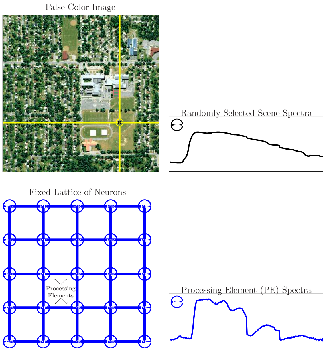
Figure 2.6: The scene spectra and the SOM PE's are both n -dimensional.
