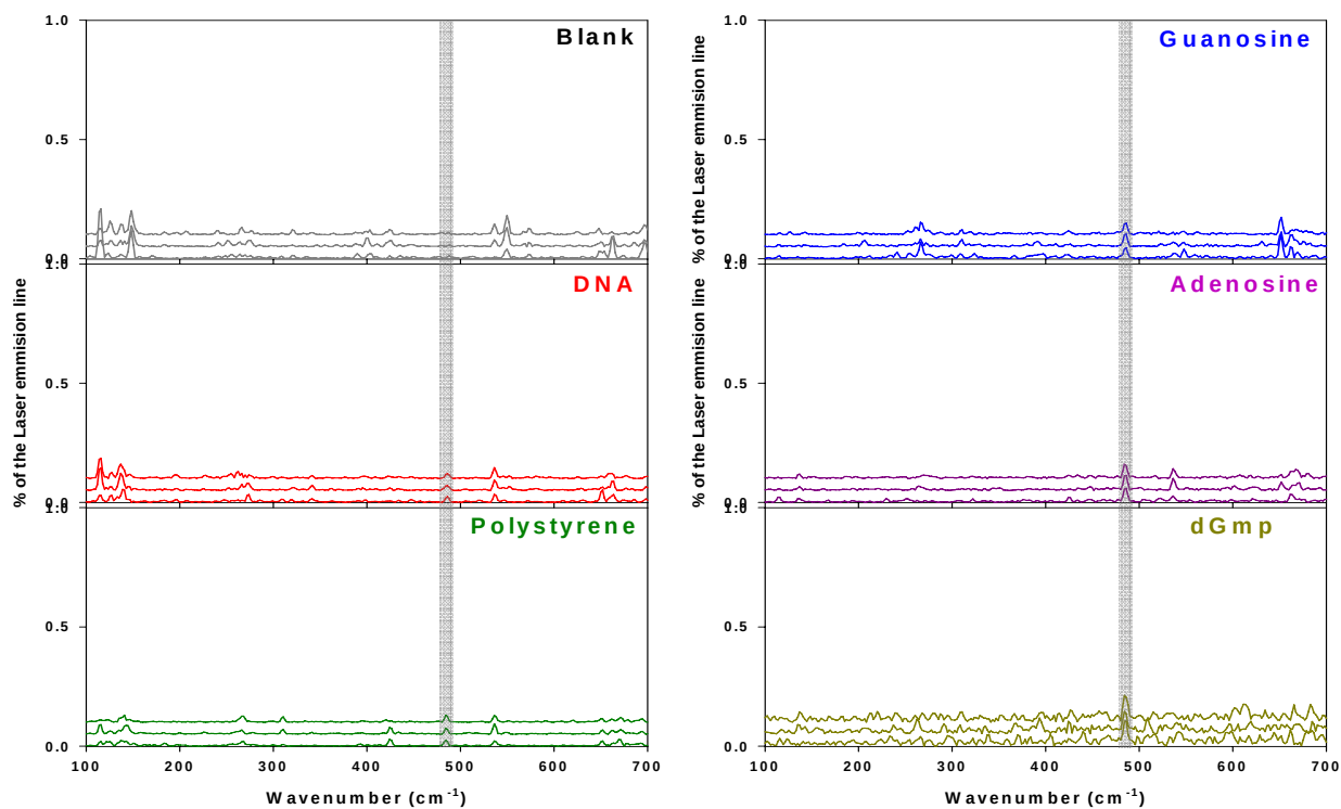
Figure 16. Emission / Transmission spectra when excited by 970 \text{cm}^{-1} \text{CO}_2 laser line. Each spectrum is average of 100 spectra.
