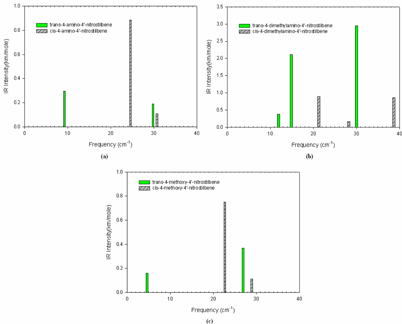
Figure 16. Very Far infrared spectrum of stilbene derivatives (<30 cm -1 ) calculated with B3LYP/6-31G(d) method in G03W and frequencies are scaled by 0.9603 to eliminate known systematic error: (a) 4-amino-4'-nitrostilbene; (b) 4-dimethylamino-4'-nitrostilbene; (c) 4-methoxy-4'-nitrostilbene.
