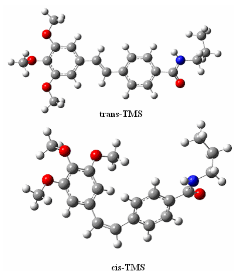
Figure 17. Geometric structure of trans- and cis- TMS
