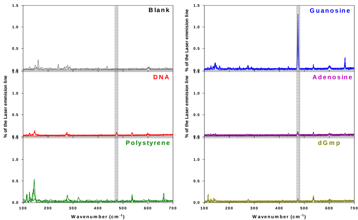
Figure 17. Emission / Transmission spectra when excited by 949 \text{cm}^{-1} \text{CO}_2 laser line. Each spectrum is average of 100 spectra.
