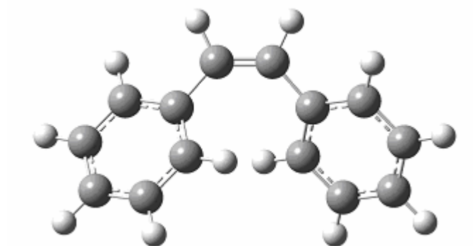
Figure 9. Geometric structure of cis-stilbene.
