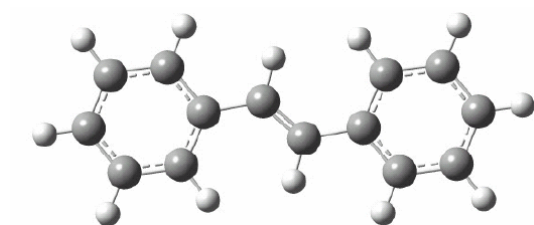
Figure 8. Geometric structure of trans-stilbene
