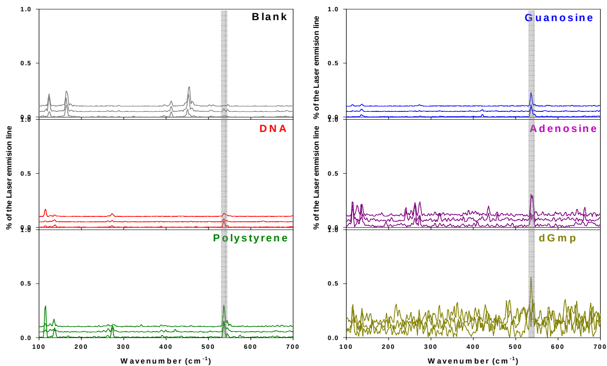
Figure 15. Emission / Transmission spectra when excited by 1080 cm -1 CO 2 laser line. Each spectrum is average of 100 spectra.
