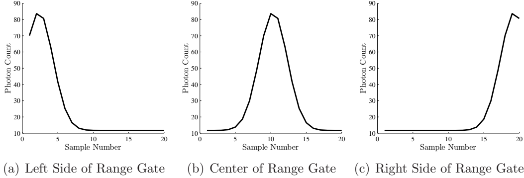
Figure 4.3: Examples of waveforms created in various positions in the range gate used in the simulated experiment.
