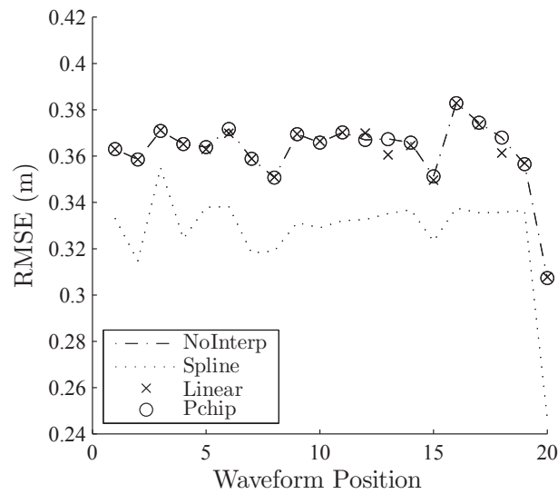
Figure 5.4: RMSE of peak estimator algorithm as waveforms change position within range gate. A 1 value for waveform position indicates a waveform on the far right side of range gate. A 20 value for waveform position indicates a waveform on the far left side of the range gate.
