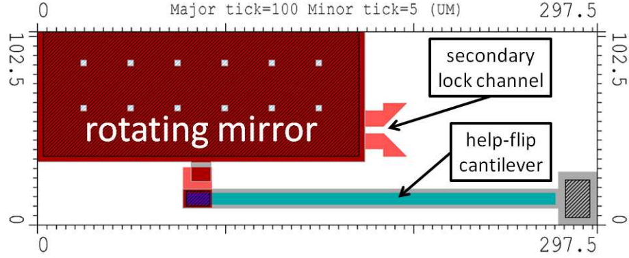
Figure 3.9: PolyMUMPs TM mirror help-flip cantilever. The Poly2-Metal stack cantilever bends upward out of the substrate plane to lift the mirror plate.
