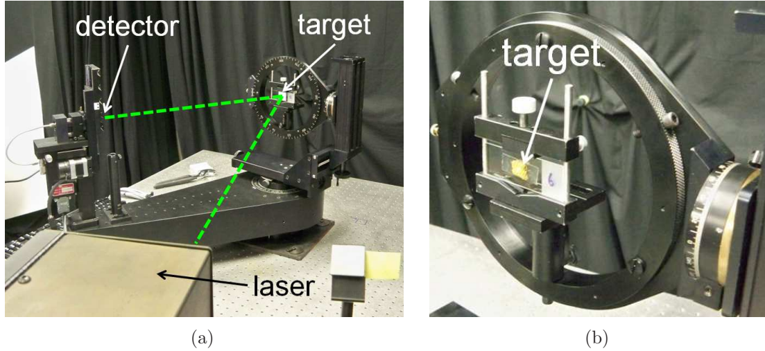
Figure 3.32: Complete Angle Scattering Instrument (CASI) BRDF measurement setup. (a) The CASI laser illuminates the target as the detector stage rotates around the sample. (b) Close up of the target stage.
