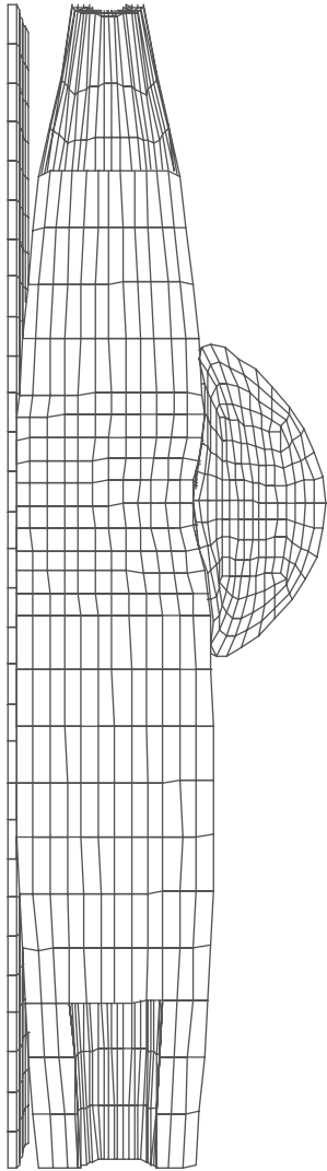
Figure 3a. Effect of 12" debris at 400 ft/s on MK 82 bomb.
