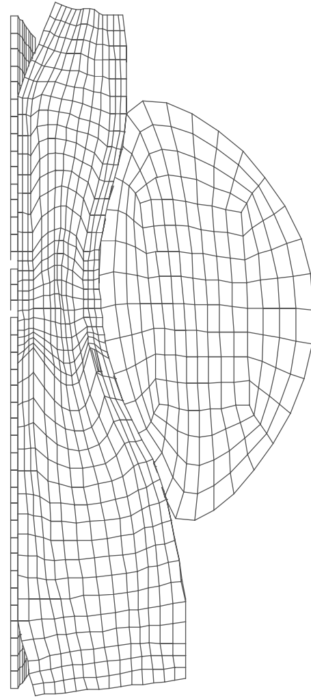
Figure 1d. Back wall and 12" debris at 1200 ft/s
