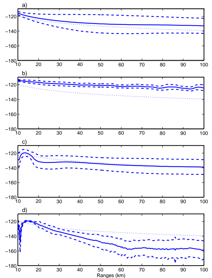
Fig. 9. The average field (solid) and plus/minus one standard deviation (dashed) based on all prior samples (a and c) and just the best posteriori samples (b and d) at 10-m height (a and b) 100-m height (c and d). For reference a r^{-1} decay (dotted) is shown on each plot.
