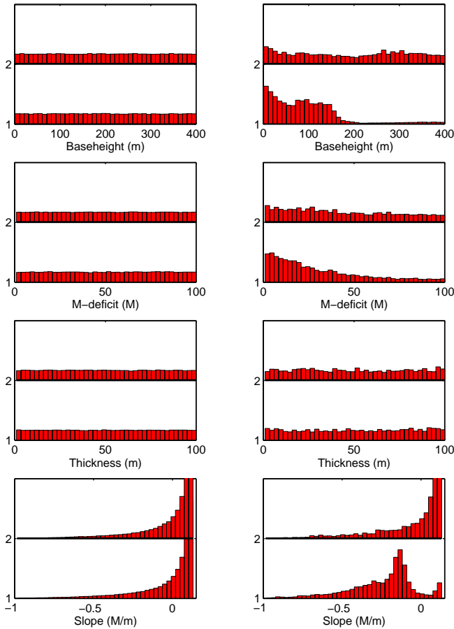
Fig. 4. Prior (left) and posterior (right) distributions of the parameter estimates.
