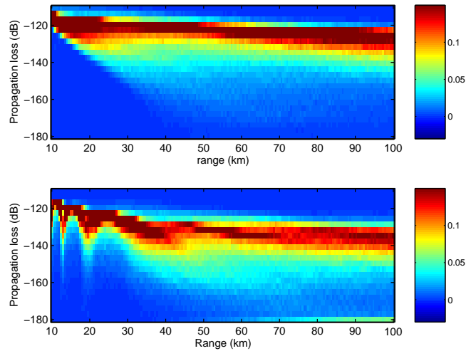
Fig. 6. Prior probability distribution for propagation loss versus range at 10 m (top) and 100 m (bottom) height.
