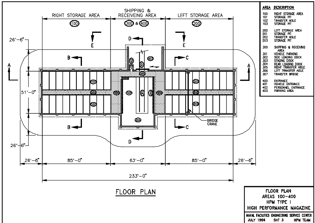
Figure 3. HP Magazine: Floor plan.
