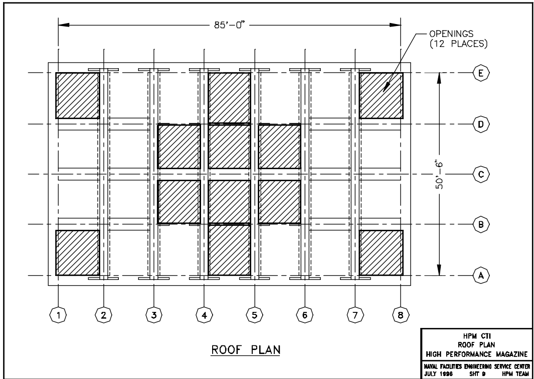
Figure 9. CT1 Structure: Roof plan.
