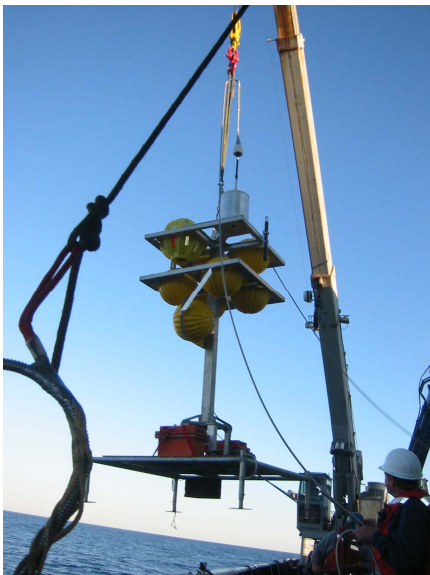
Figure 2: Nov 04- Elevator showing fiber pack at top
