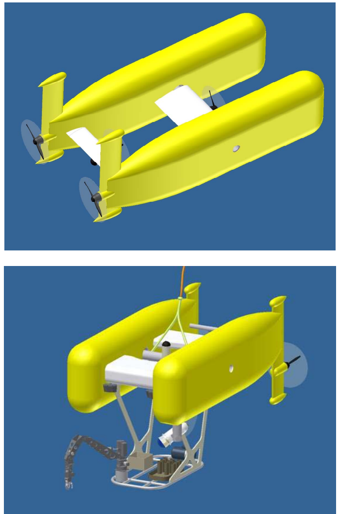
Figure 1: HROV in the autonomous and remotely operated configurations
