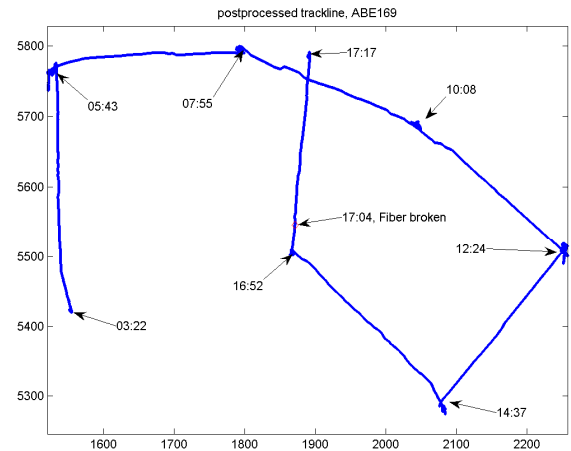
Figure 4: Path followed by ABE on Dive 4
