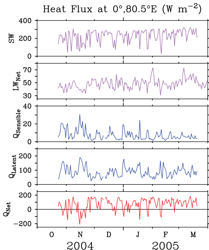
Fig. 4. Short wave, net long wave, sensible, latent and net surface heat flux measured and computed from an ATLAS mooring near 0° 80°E in the Indian Ocean.
