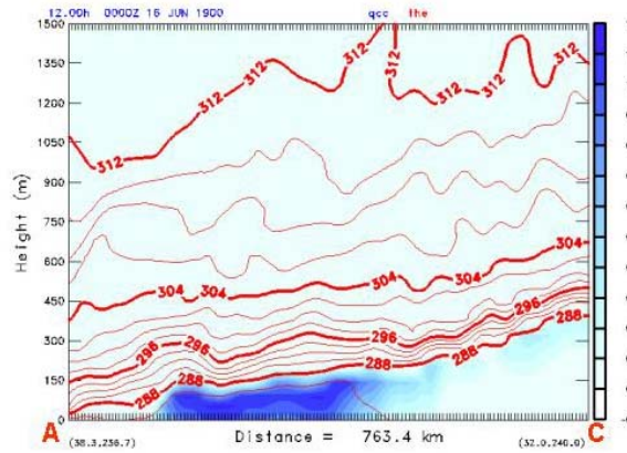
Figure 5. Cross section of potential temperature (K) and cloud water mixing ratio (gm/Kg; shaded) in the plane A-C.
