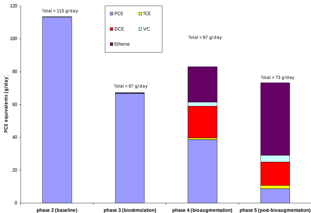
Figure 5. Mass Discharge by Phase Calculated from Data Collected During Major Sampling Events.
