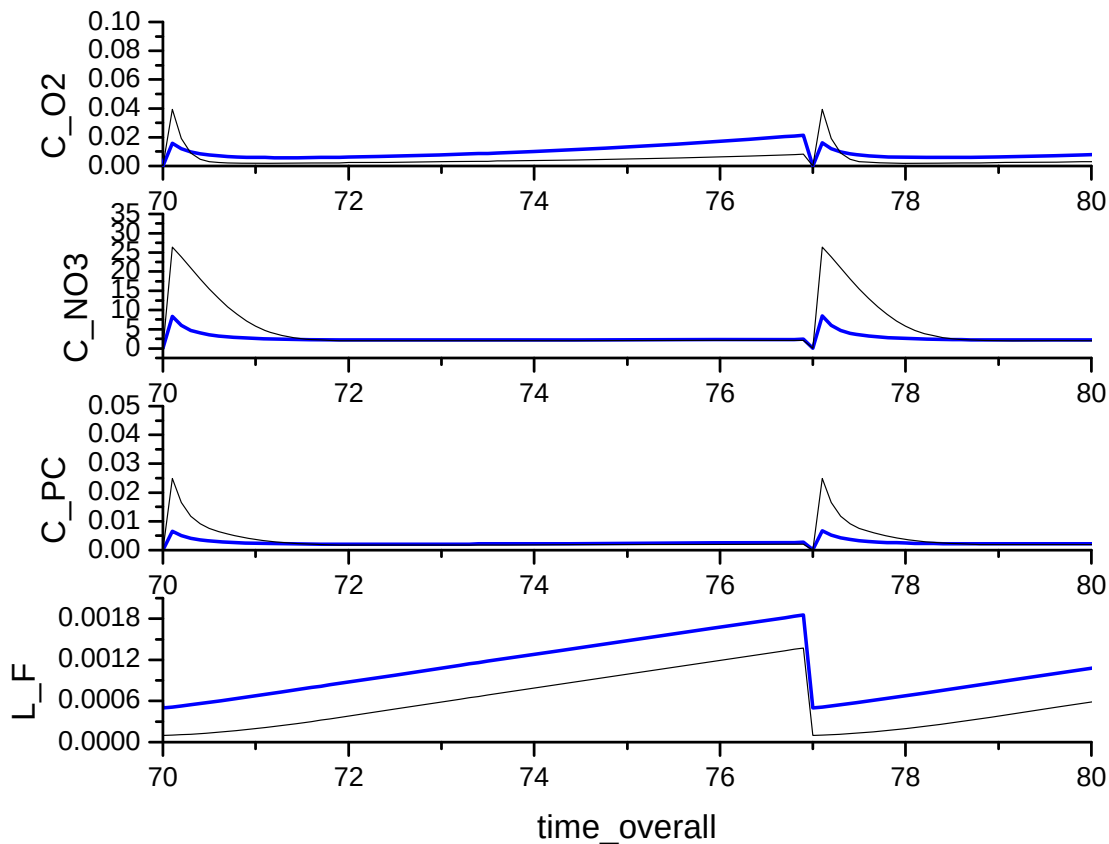
Figure E.12 - Comparison of the Influence of the Base Thickness of 100 µm (black line) and 500 µm (thick blue line) for a Backwashing Interval of 7 d.
