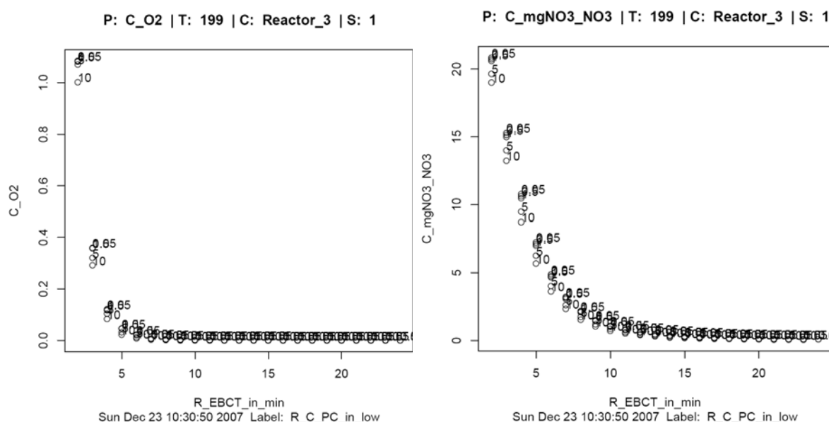
Figure E.15 - Effluent Oxygen and Nitrate Concentrations for Different EBCT (x-axis) Simulated for a Range of Influent Perchlorate Concentrations (number in plot in mg/L, 0.05 – 10 mg/L). Otherwise Standard Conditions (D/A ratio = 1.8, parameter combination #14).
