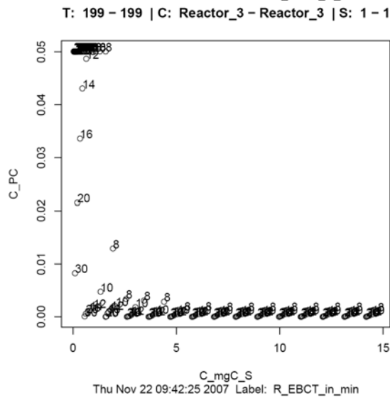
Figure E.9 - Correlation of Effluent Perchlorate Concentration with Effluent Oxygen (top), Nitrate (middle), and Organic Substrate (bottom) Concentrations for all [D/A] with EBCT (numbers in plot in min) for Influent Perchlorate Concentrations of 50 µg/L.
