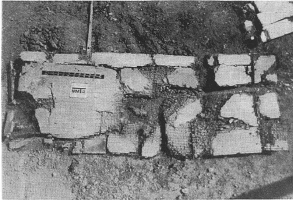
Figure 13. Post - test view of roof slab: Test 11.
