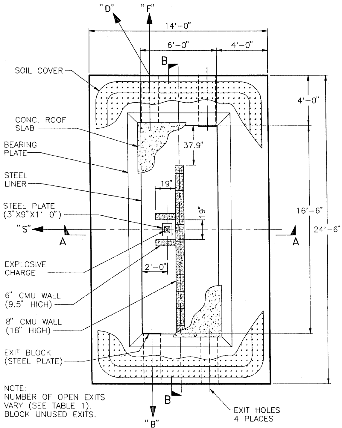
FIGURE 2a. TEST FIXTURE: PLAN VIEW
