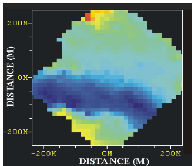
Fig. 4. Plot of gridded temperature at 1500 m depth, western North Atlantic Ocean, March 2003.
